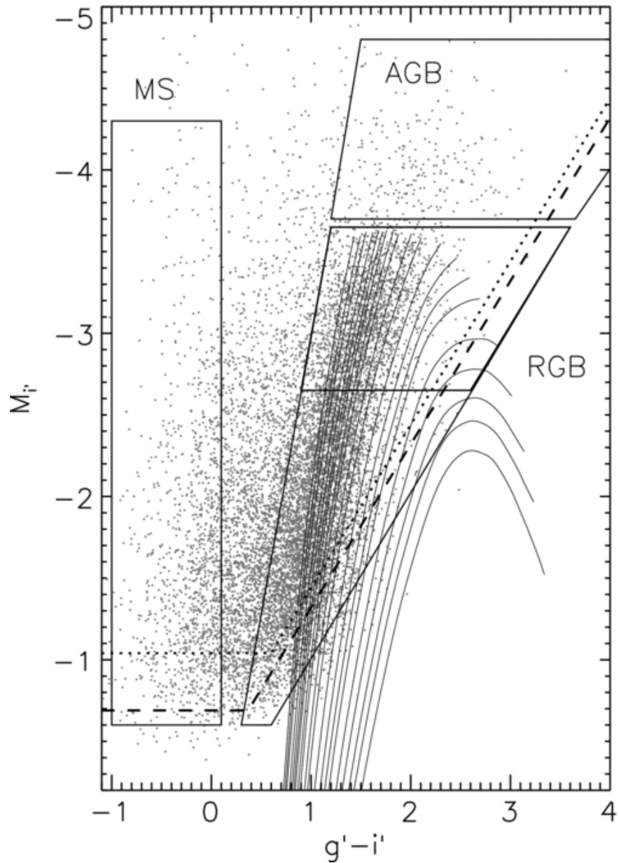
Figure 4. from The Structure and Metallicity Gradient in the Extreme Outer Disk of NGC 7793 Vlaji, Bland-Hawthorn, & Freeman 2011 ApJ 732 7 doi:10.1088/0004-637X/732/1/7 https://dx.doi.org/10.1088/0004-637X/732/1/7
