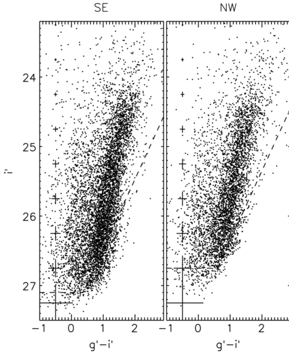
Figure 3. from The Structure and Metallicity Gradient in the Extreme Outer Disk of NGC 7793 Vlaji, Bland-Hawthorn, & Freeman 2011 ApJ 732 7 doi:10.1088/0004-637X/732/1/7 https://dx.doi.org/10.1088/0004-637X/732/1/7 © 2011. The American Astronomical Society. All rights reserved.
