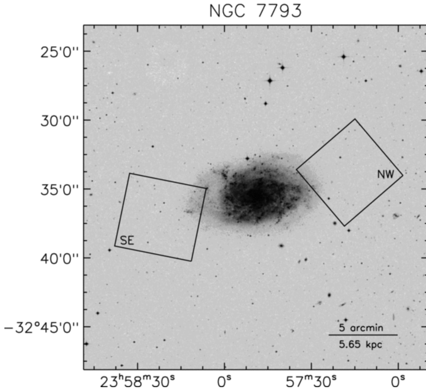
Figure 1. from The Structure and Metallicity Gradient in the Extreme Outer Disk of NGC 7793 Vlaji, Bland-Hawthorn, & Freeman 2011 ApJ 732 7 doi:10.1088/0004-637X/732/1/7 https://dx.doi.org/10.1088/0004-637X/732/1/7 © 2011. The American Astronomical Society. All rights reserved.
