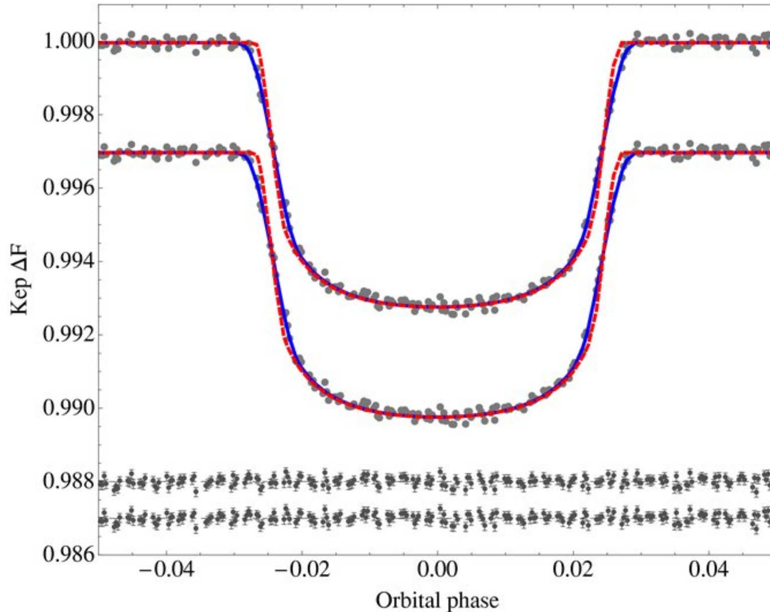
Figure 6. from An Independent Analysis of Kepler-4b Through Kepler-8b Kipping & Bakos 2011 ApJ 730 50 doi:10.1088/0004-637X/730/1/50 https://dx.doi.org/10.1088/0004-637X/730/1/50 © 2011. The American Astronomical Society. All rights reserved.
