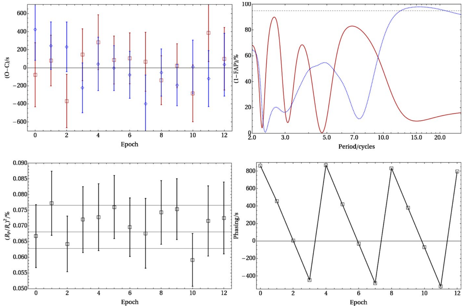
Figure 5. from An Independent Analysis of Kepler-4b Through Kepler-8b Kipping & Bakos 2011 ApJ 730 50 doi:10.1088/0004-637X/730/1/50 https://dx.doi.org/10.1088/0004-637X/730/1/50 © 2011. The American Astronomical Society. All rights reserved.
