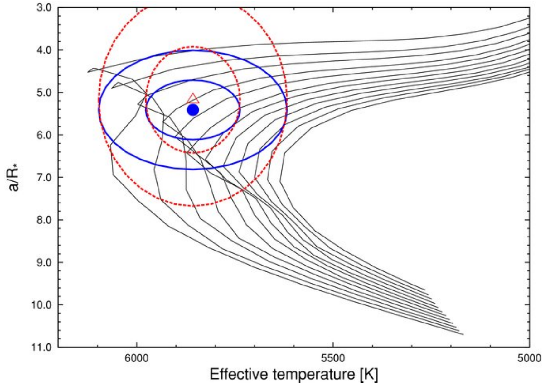
Figure 4. from An Independent Analysis of Kepler-4b Through Kepler-8b Kipping & Bakos 2011 ApJ 730 50 doi:10.1088/0004-637X/730/1/50 https://dx.doi.org/10.1088/0004-637X/730/1/50 © 2011. The American Astronomical Society. All rights reserved.
