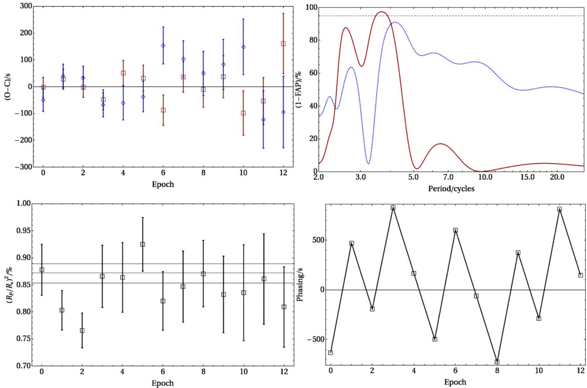
Figure 26. from An Independent Analysis of Kepler-4b Through Kepler-8b Kipping & Bakos 2011 ApJ 730 50 doi:10.1088/0004-637X/730/1/50 https://dx.doi.org/10.1088/0004-637X/730/1/50 © 2011. The American Astronomical Society. All rights reserved.
