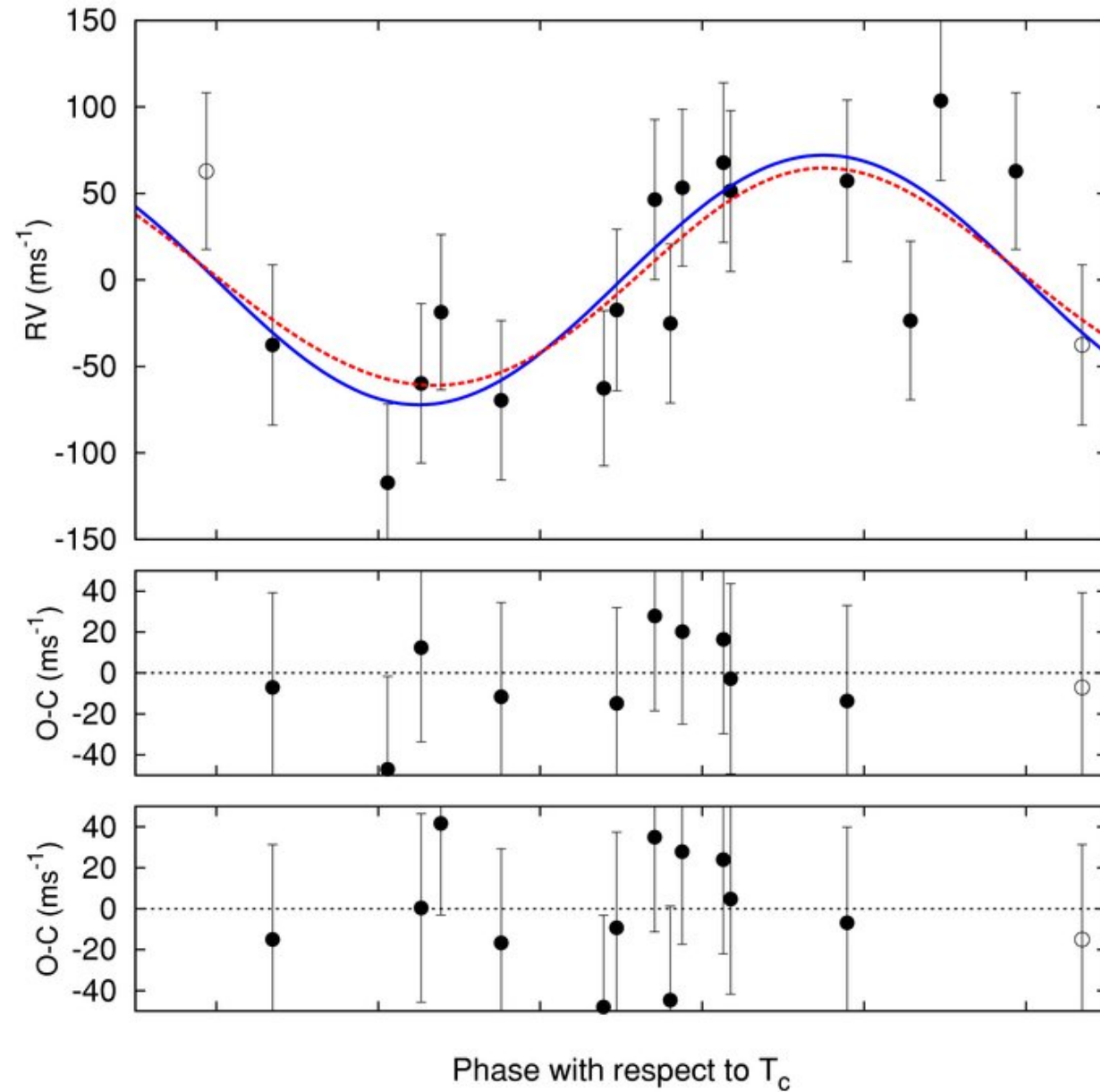
Figure 24. from An Independent Analysis of Kepler-4b Through Kepler-8b Kipping & Bakos 2011 ApJ 730 50 doi:10.1088/0004-637X/730/1/50 https://dx.doi.org/10.1088/0004-637X/730/1/50 © 2011. The American Astronomical Society. All rights reserved.
