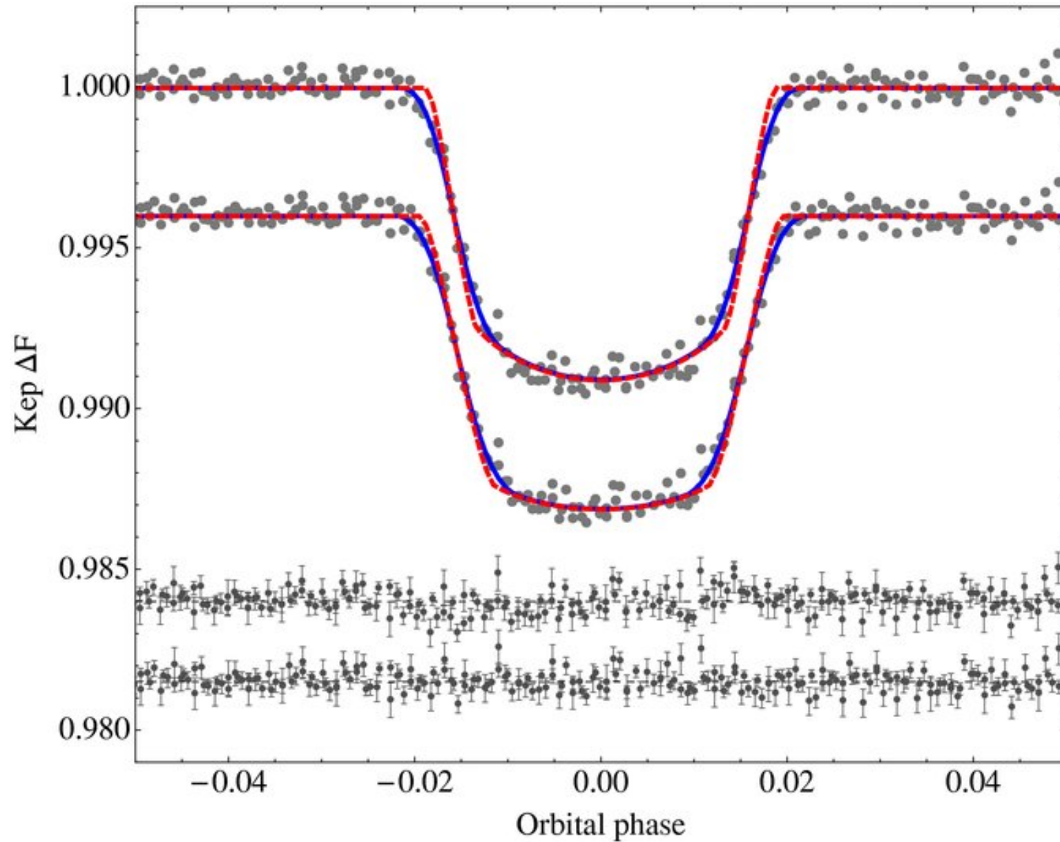
Figure 23. from An Independent Analysis of Kepler-4b Through Kepler-8b Kipping & Bakos 2011 ApJ 730 50 doi:10.1088/0004-637X/730/1/50 https://dx.doi.org/10.1088/0004-637X/730/1/50 © 2011. The American Astronomical Society. All rights reserved.
