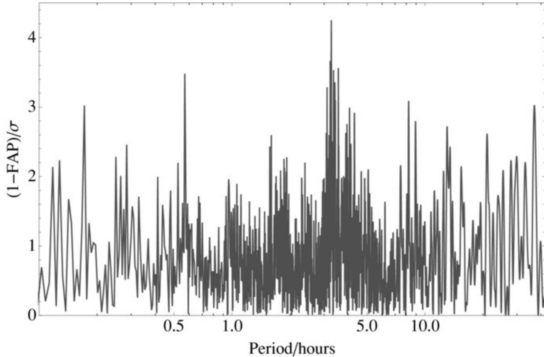
Figure 22. from An Independent Analysis of Kepler-4b Through Kepler-8b Kipping & Bakos 2011 ApJ 730 50 doi:10.1088/0004-637X/730/1/50 https://dx.doi.org/10.1088/0004-637X/730/1/50 © 2011. The American Astronomical Society. All rights reserved.
