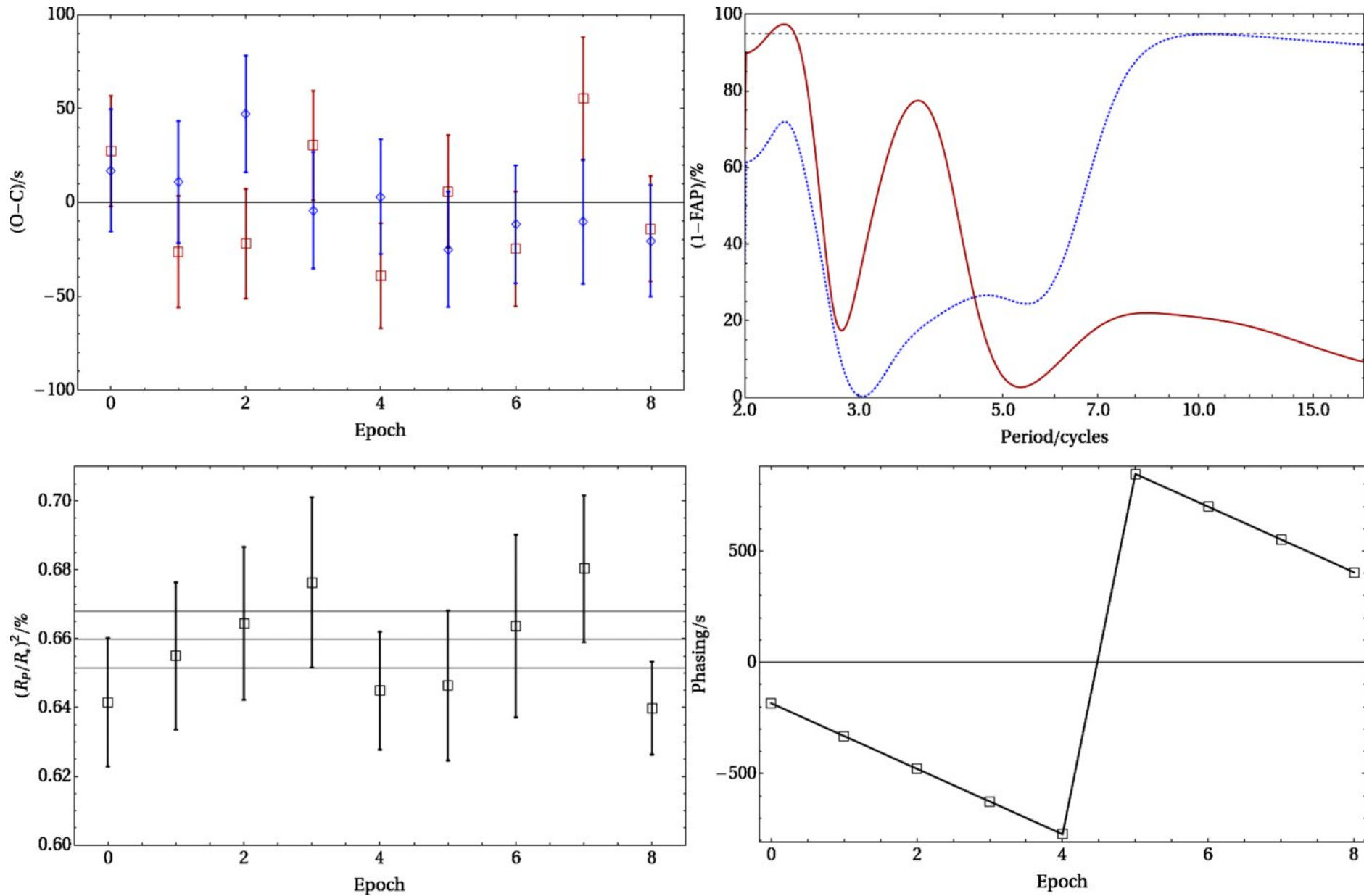
Figure 21. from An Independent Analysis of Kepler-4b Through Kepler-8b Kipping & Bakos 2011 ApJ 730 50 doi:10.1088/0004-637X/730/1/50 https://dx.doi.org/10.1088/0004-637X/730/1/50 © 2011. The American Astronomical Society. All rights reserved.
