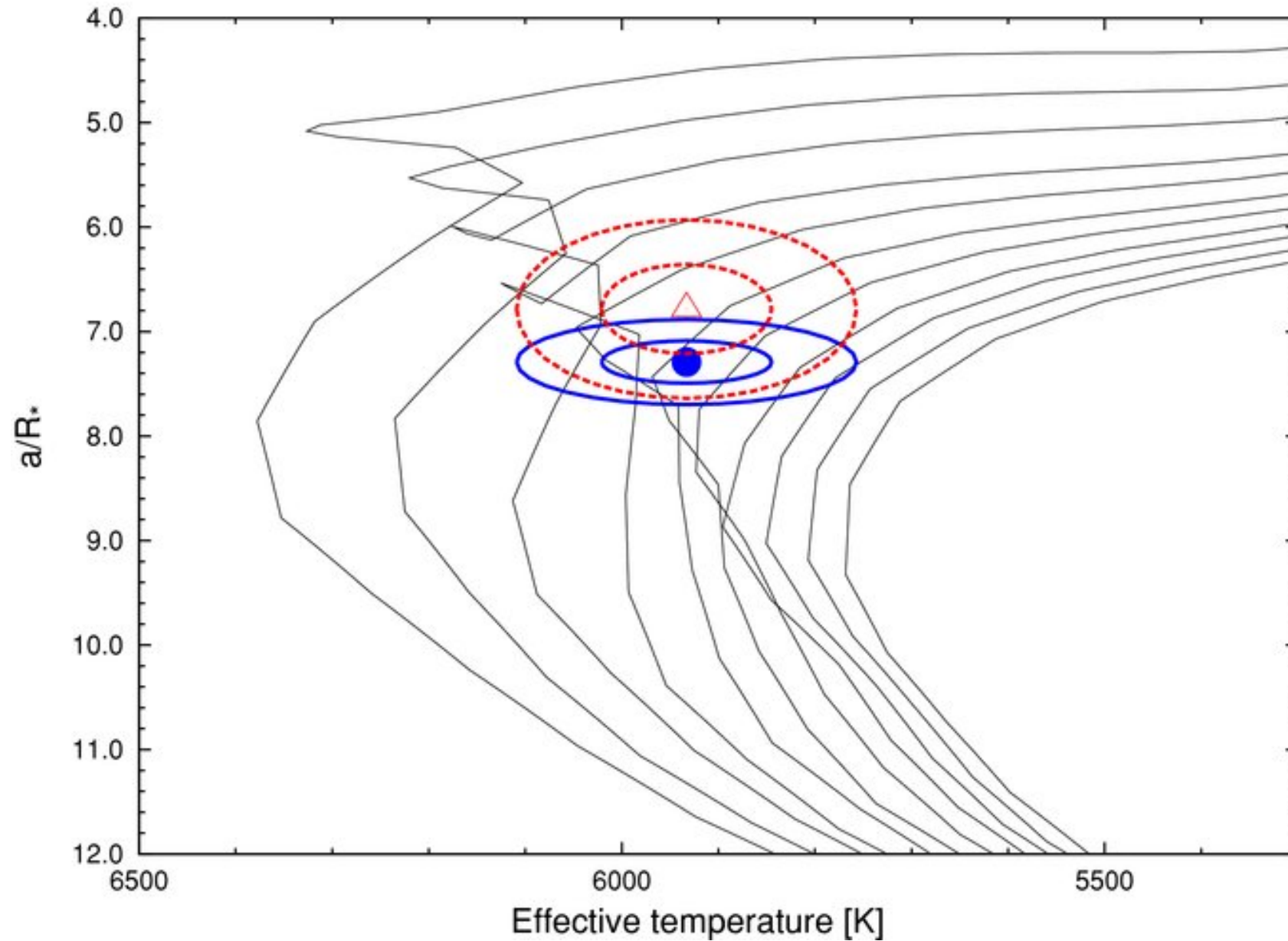
Figure 20. from An Independent Analysis of Kepler-4b Through Kepler-8b Kipping & Bakos 2011 ApJ 730 50 doi:10.1088/0004-637X/730/1/50 https://dx.doi.org/10.1088/0004-637X/730/1/50 © 2011. The American Astronomical Society. All rights reserved.
