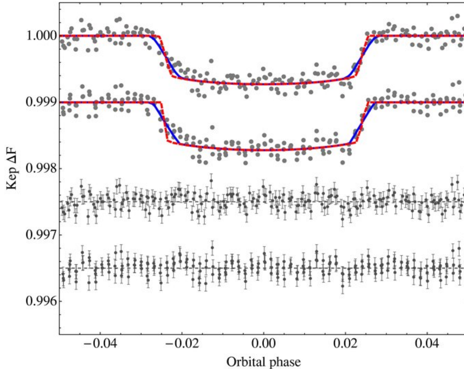
Figure 2. from An Independent Analysis of Kepler-4b Through Kepler-8b Kipping & Bakos 2011 ApJ 730 50 doi:10.1088/0004-637X/730/1/50 https://dx.doi.org/10.1088/0004-637X/730/1/50 © 2011. The American Astronomical Society. All rights reserved.
