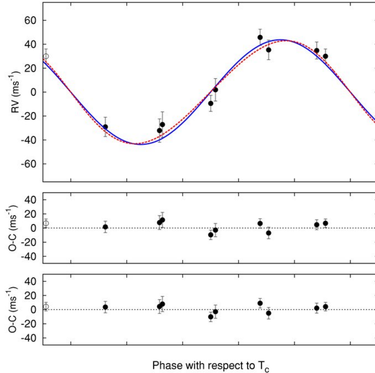
Figure 18. from An Independent Analysis of Kepler-4b Through Kepler-8b Kipping & Bakos 2011 ApJ 730 50 doi:10.1088/0004-637X/730/1/50 https://dx.doi.org/10.1088/0004-637X/730/1/50 © 2011. The American Astronomical Society. All rights reserved.
