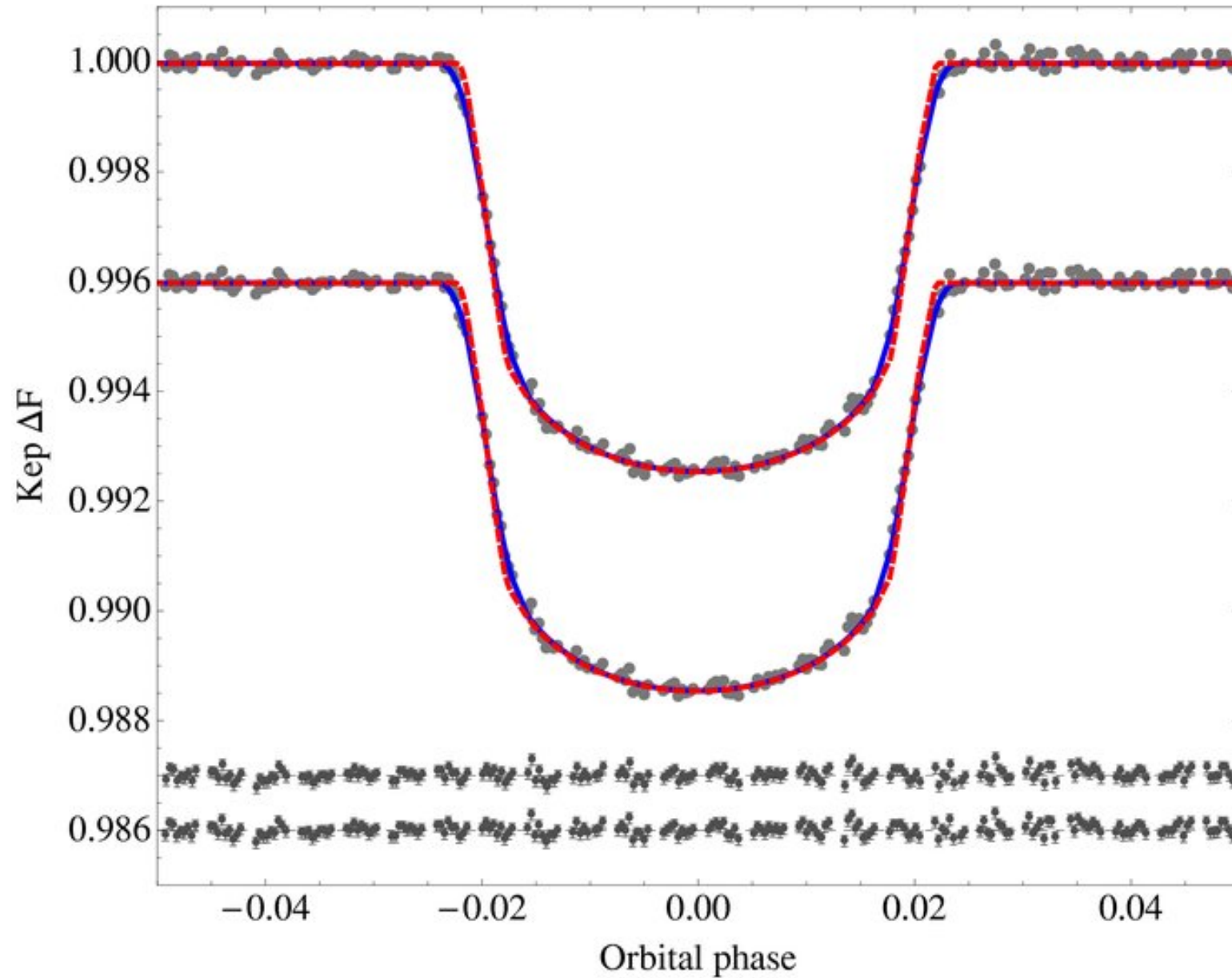
Figure 16. from An Independent Analysis of Kepler-4b Through Kepler-8b Kipping & Bakos 2011 ApJ 730 50 doi:10.1088/0004-637X/730/1/50 https://dx.doi.org/10.1088/0004-637X/730/1/50 © 2011. The American Astronomical Society. All rights reserved.
