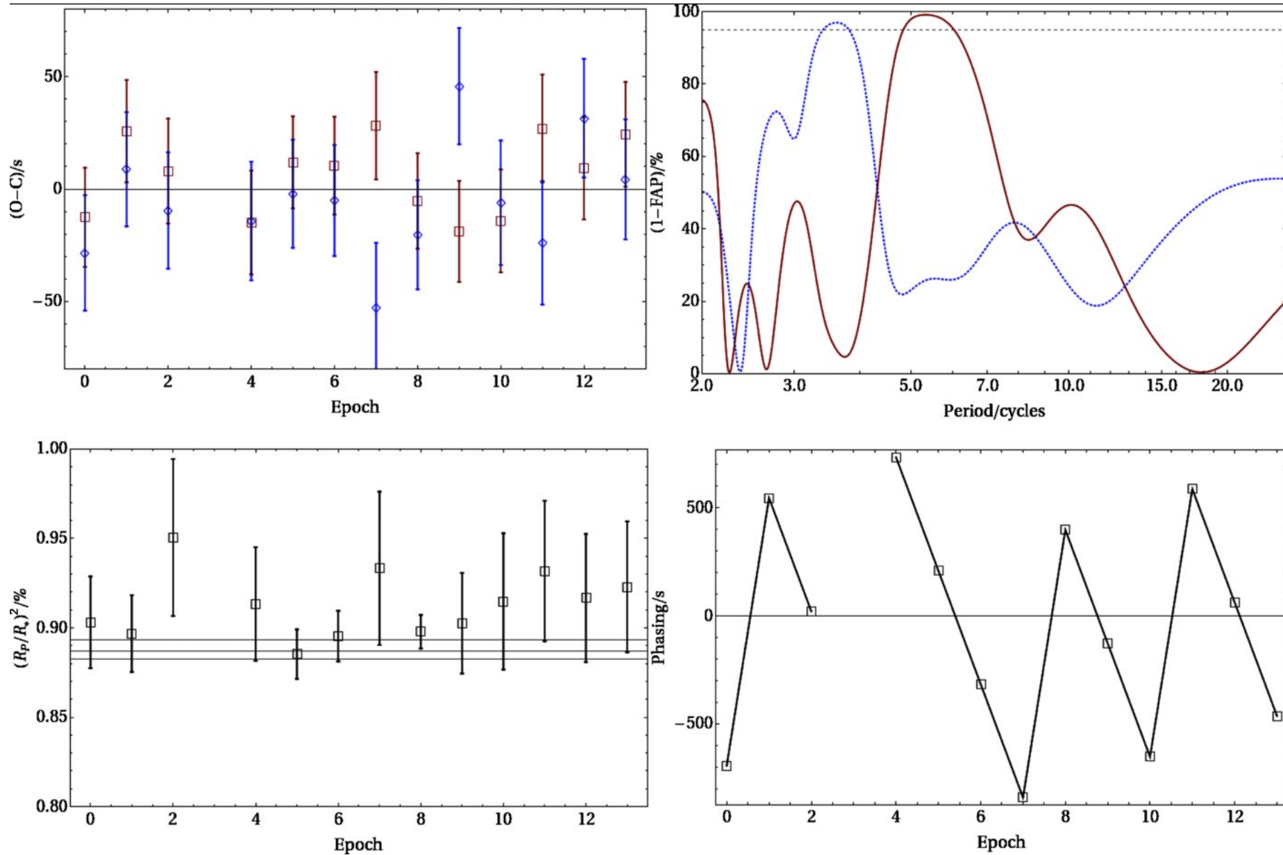
Figure 15. from An Independent Analysis of Kepler-4b Through Kepler-8b Kipping & Bakos 2011 ApJ 730 50 doi:10.1088/0004-637X/730/1/50 https://dx.doi.org/10.1088/0004-637X/730/1/50 © 2011. The American Astronomical Society. All rights reserved.
