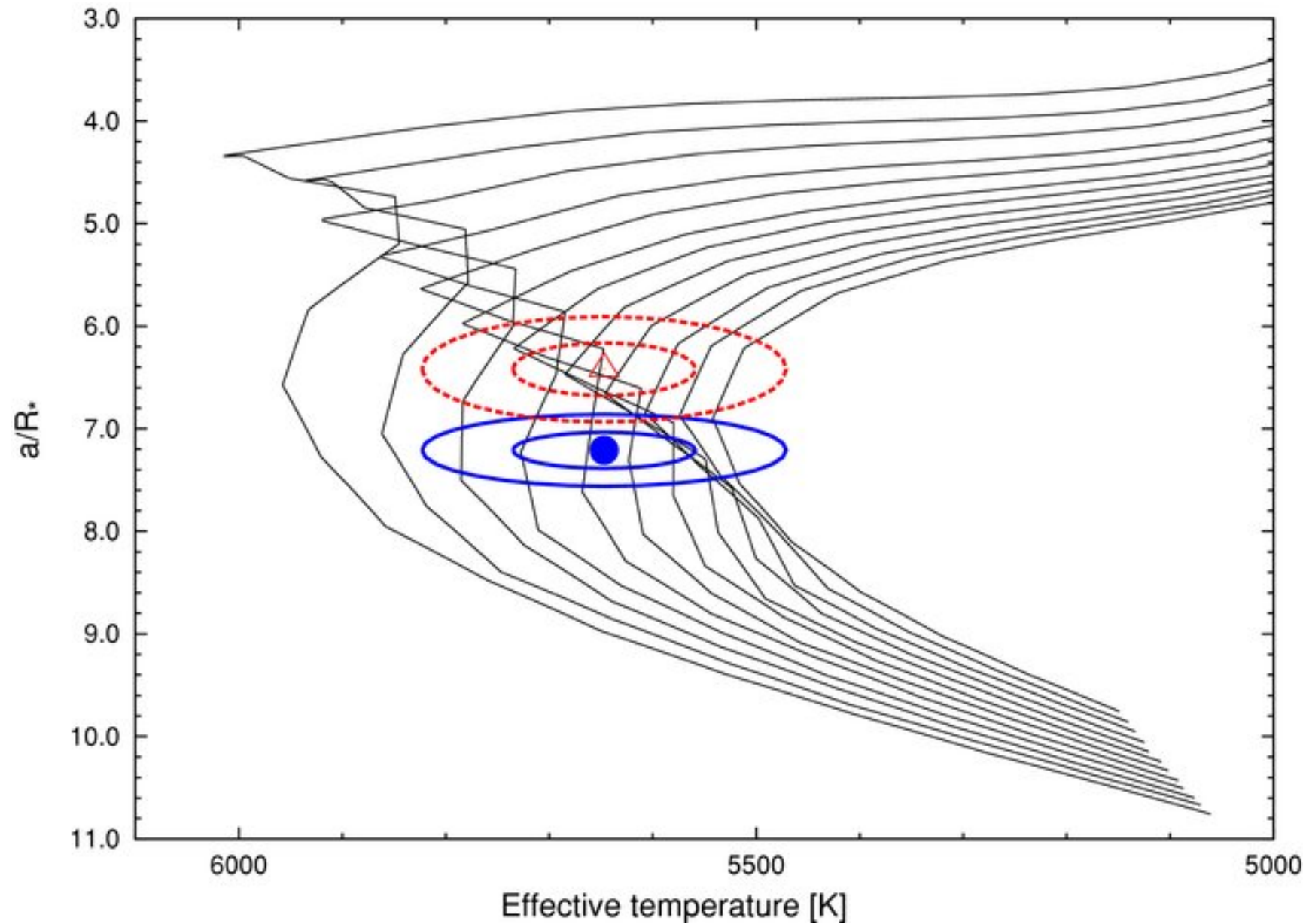
Figure 14. from An Independent Analysis of Kepler-4b Through Kepler-8b Kipping & Bakos 2011 ApJ 730 50 doi:10.1088/0004-637X/730/1/50 https://dx.doi.org/10.1088/0004-637X/730/1/50 © 2011. The American Astronomical Society. All rights reserved.
