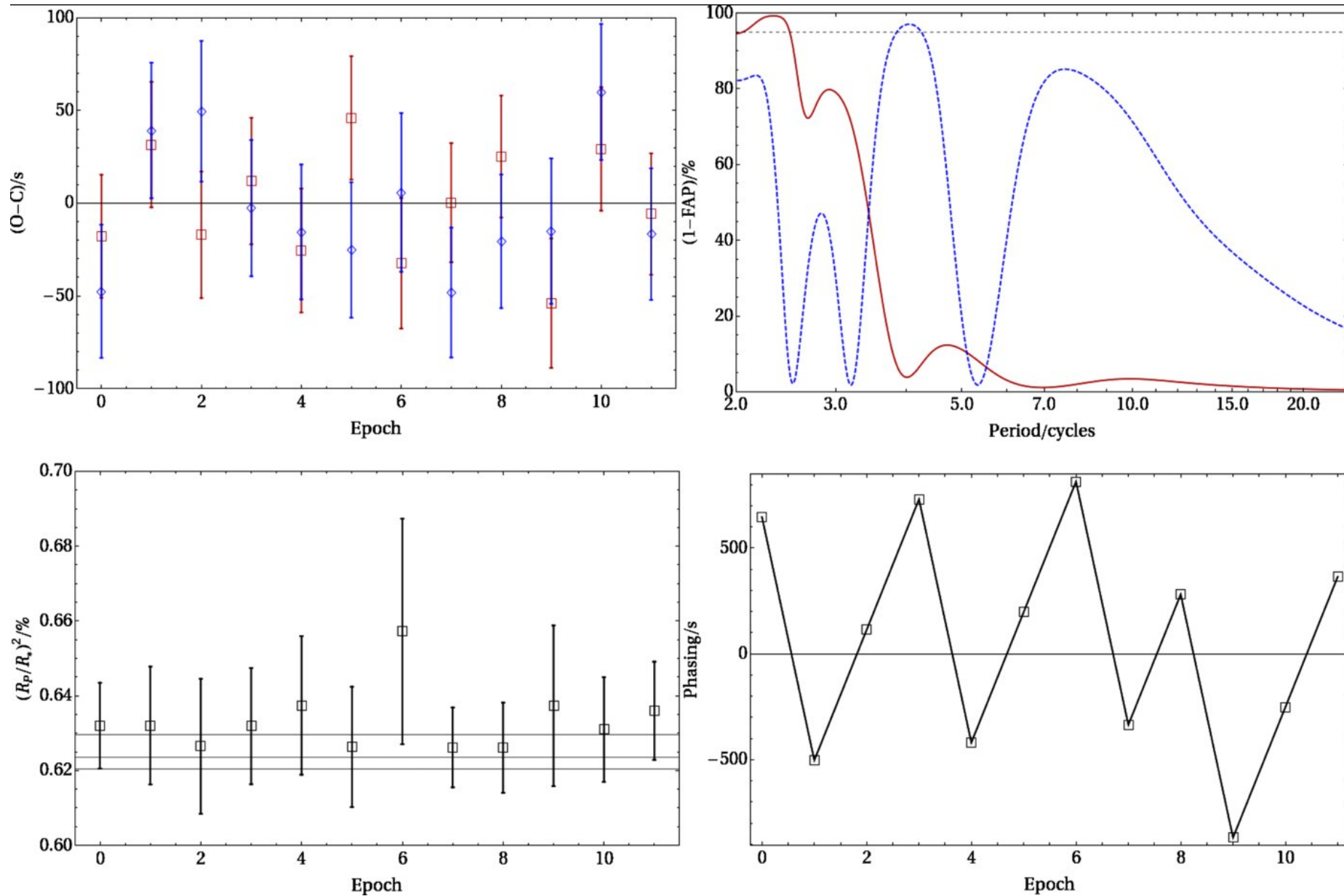
Figure 11. from An Independent Analysis of Kepler-4b Through Kepler-8b Kipping & Bakos 2011 ApJ 730 50 doi:10.1088/0004-637X/730/1/50 https://dx.doi.org/10.1088/0004-637X/730/1/50 © 2011. The American Astronomical Society. All rights reserved.
