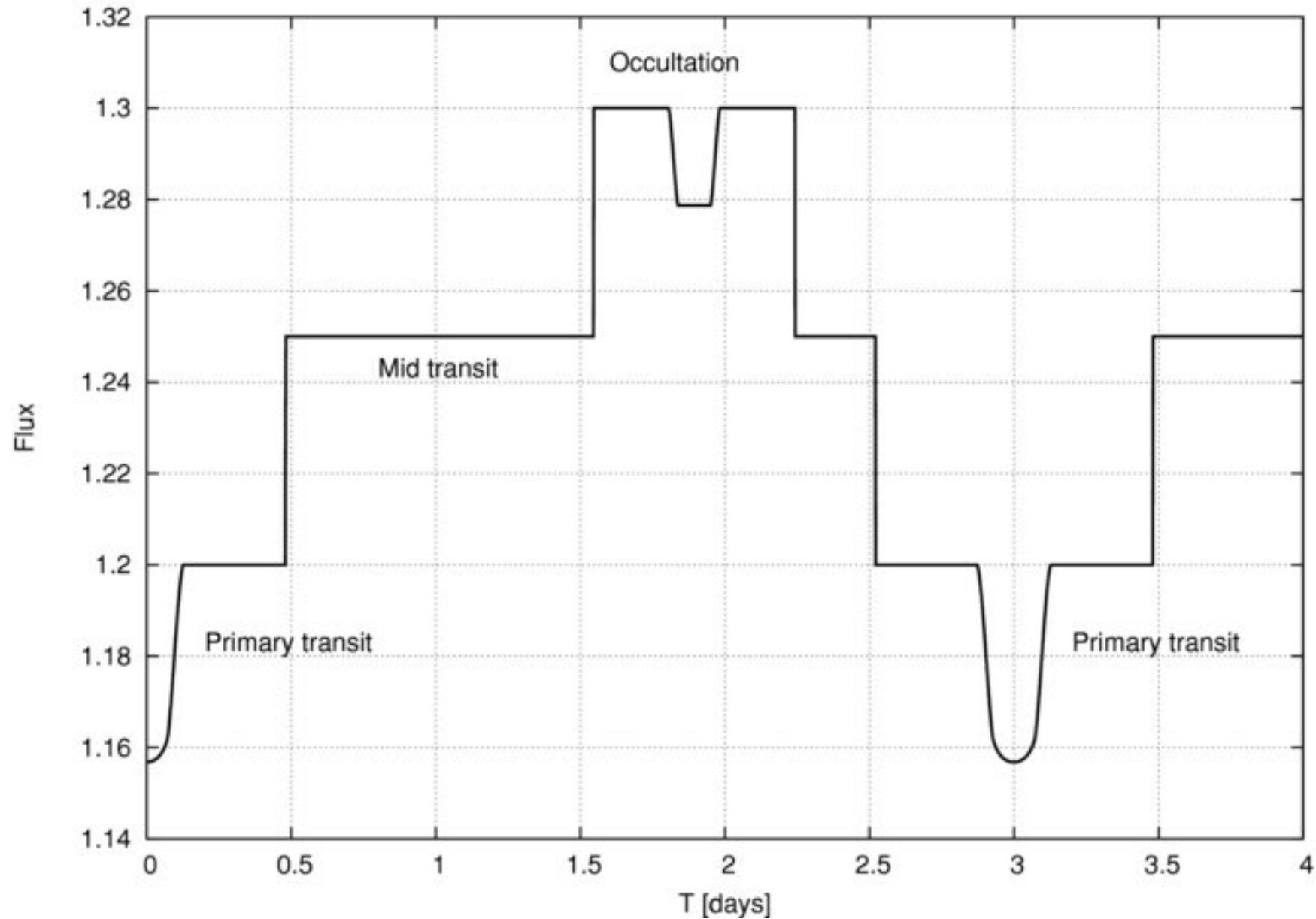
Figure 1. from An Independent Analysis of Kepler-4b Through Kepler-8b Kipping & Bakos 2011 ApJ 730 50 doi:10.1088/0004-637X/730/1/50 https://dx.doi.org/10.1088/0004-637X/730/1/50 © 2011. The American Astronomical Society. All rights reserved.
