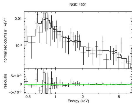
(k) Chandra spectrum.
