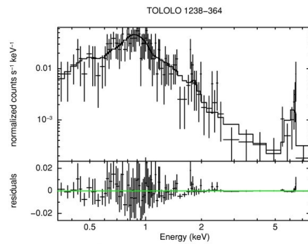
(l) Chandra spectrum.
