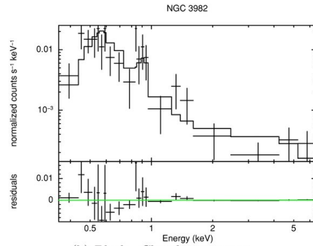
(h) Black - Chandra spectrum.
