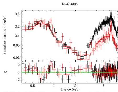
(i) Black - XMM PN spectrum from December 2002 observation, red - XMM PN spectrum from July 2002 observation.
