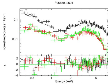
(g) Black - XMM PN spectrum, red - Chandra spectrum from 2001 observation, green - Chandra spectrum from 2002 observation.
