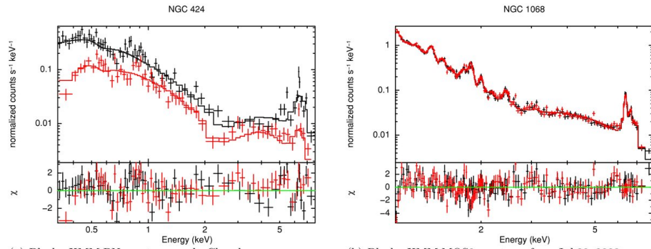
(a) Black - XMM PN spectrum, red - Chandra spectrum
