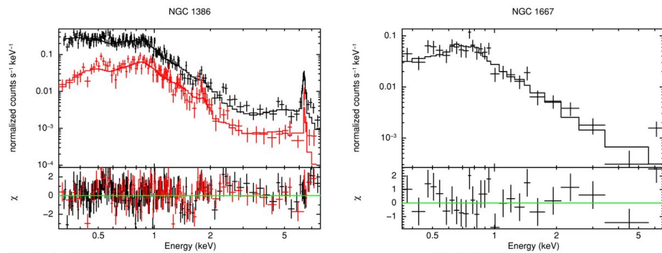
(e) Black - XMM PN spectrum, red - Chandra spectrum.
