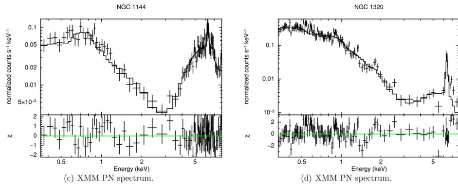
(c) XMM PN spectrum.
