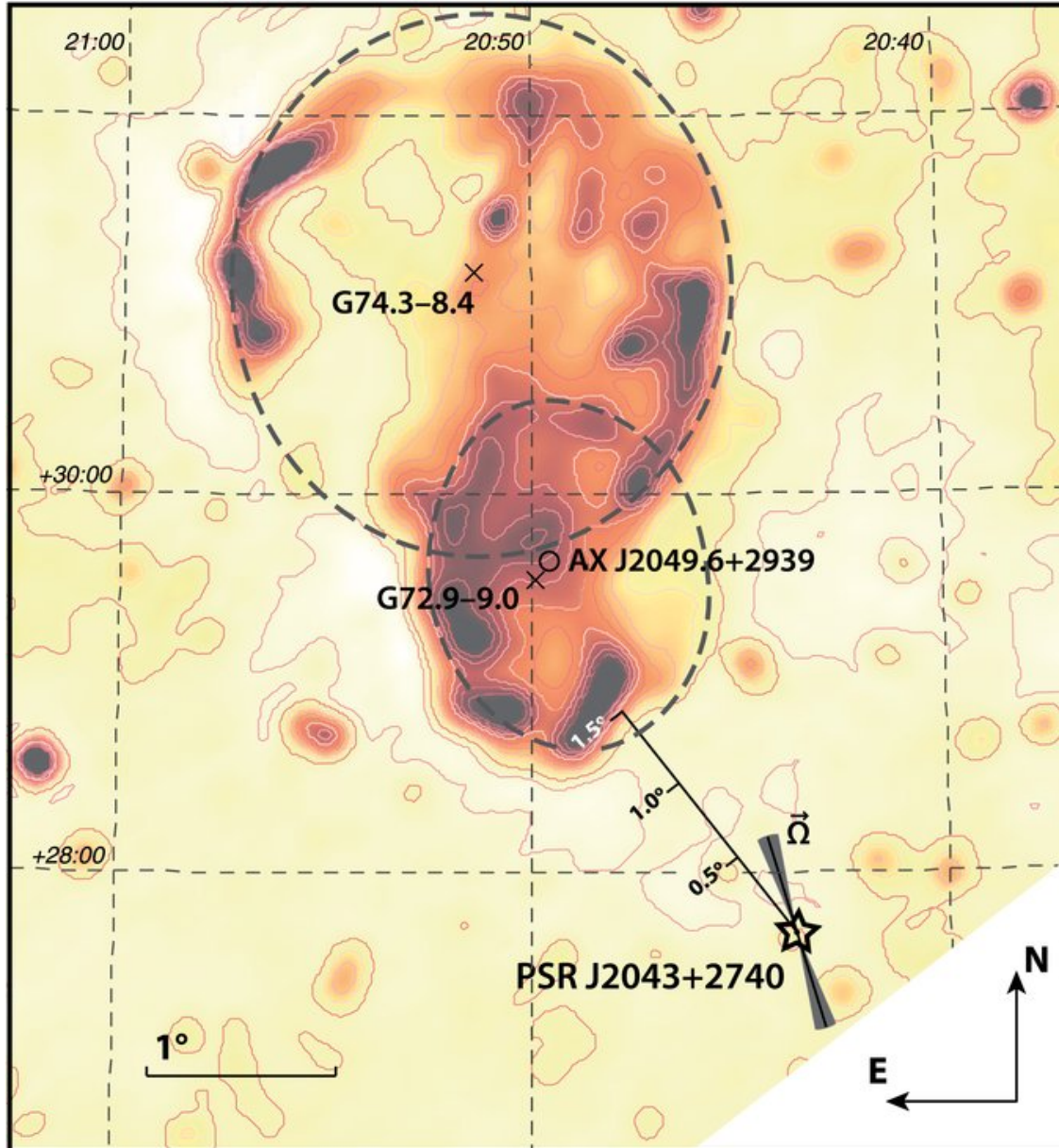
Figure 6. from Radio and -ray Constraints on the Emission Geometry and Birthplace of PSR J2043+2740 Noutsos et al. 2011 ApJ 728 77 doi:10.1088/0004-637X/728/2/77 https://dx.doi.org/10.1088/0004-637X/728/2/77 © 2011. The American Astronomical Society. All rights reserved.
