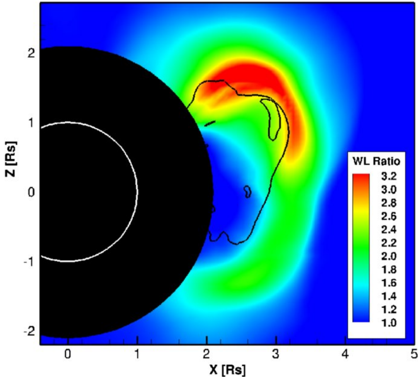
Figure 5. from Evolution of Piled-up Compressions in Modeled Coronal Mass Ejection Sheaths and the Resulting Sheath Structures Das et al. 2011 ApJ 729 112 doi:10.1088/0004-637X/729/2/112 https://dx.doi.org/10.1088/0004-637X/729/2/112 © 2011. The American Astronomical Society. All rights reserved.
