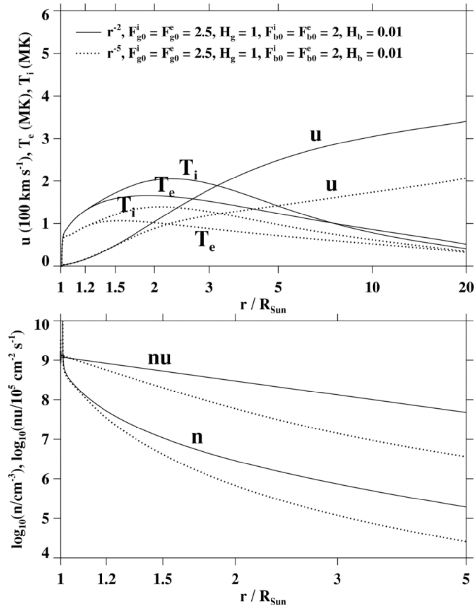
Figure 5. from Two-temperature Models for Polar Plumes: Cooling by Means of Strong Base Heating Grappin, Wang, & Pantellini 2011 ApJ 727 30 doi:10.1088/0004-637X/727/1/30 https://dx.doi.org/10.1088/0004-637X/727/1/30
