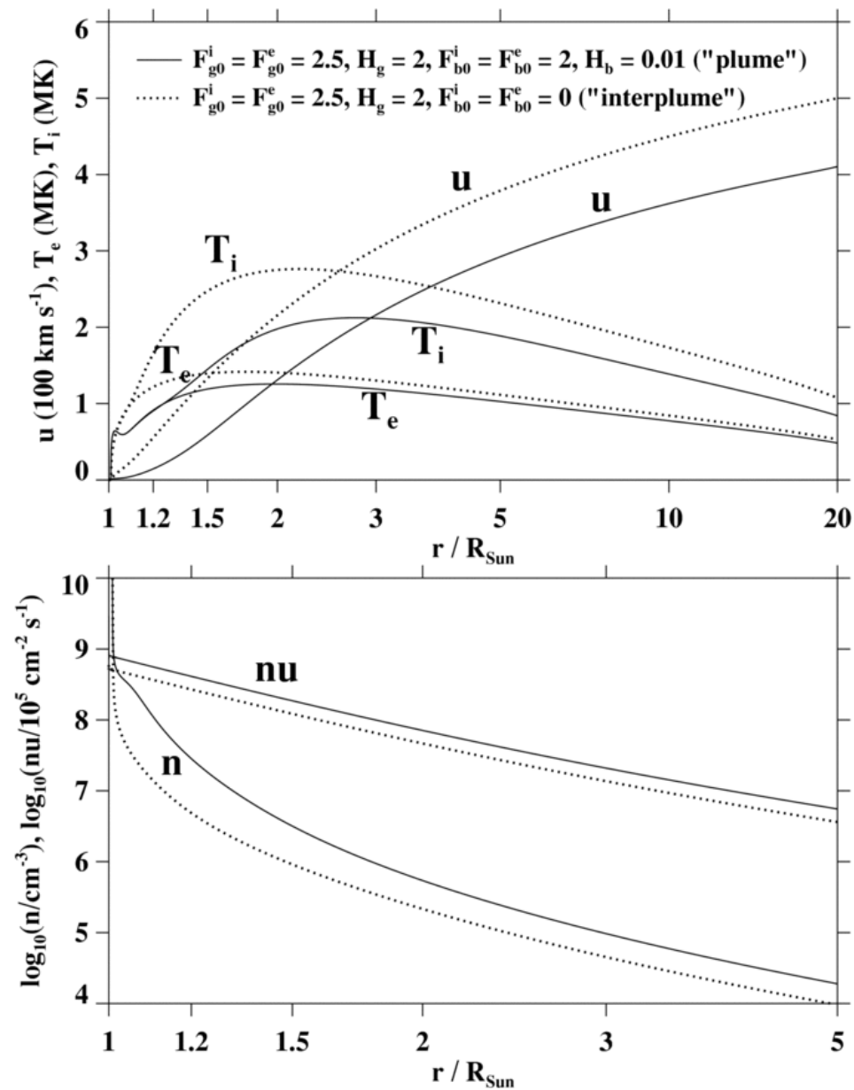
Figure 4. from Two-temperature Models for Polar Plumes: Cooling by Means of Strong Base Heating Grappin, Wang, & Pantellini 2011 ApJ 727 30 doi:10.1088/0004-637X/727/1/30 https://dx.doi.org/10.1088/0004-637X/727/1/30
