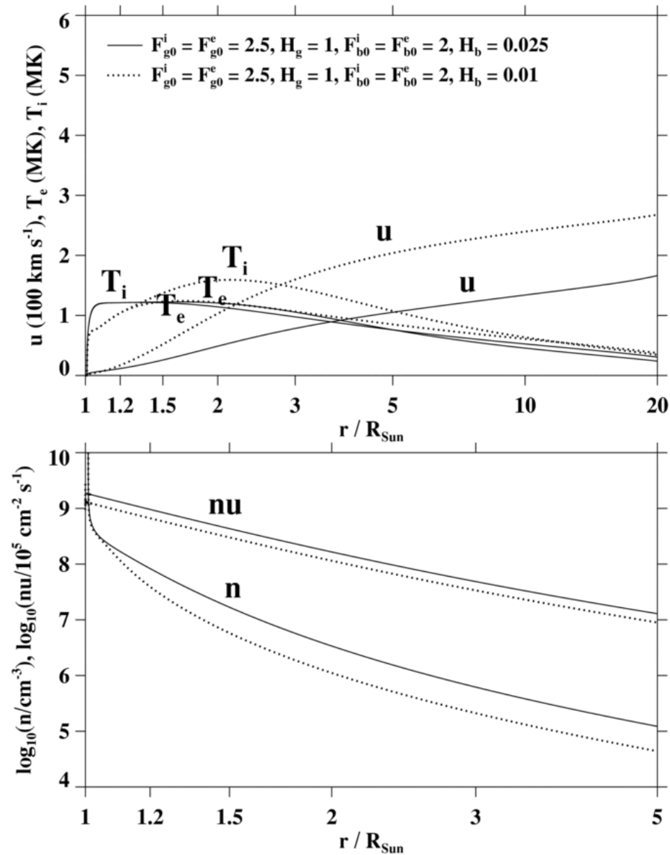
Figure 3. from Two-temperature Models for Polar Plumes: Cooling by Means of Strong Base Heating Grappin, Wang, & Pantellini 2011 ApJ 727 30 doi:10.1088/0004-637X/727/1/30 https://dx.doi.org/10.1088/0004-637X/727/1/30
