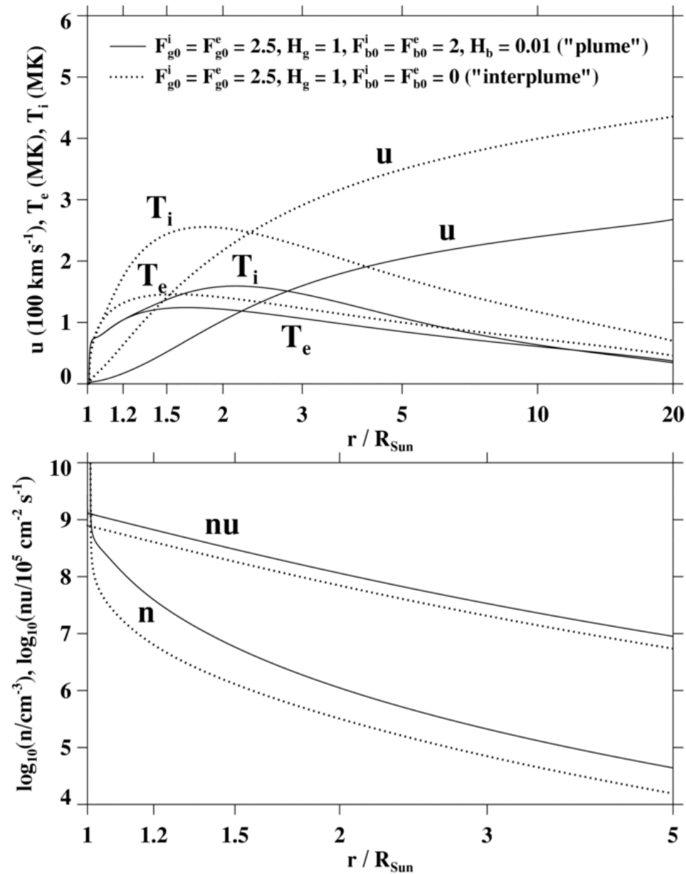
Figure 2. from Two-temperature Models for Polar Plumes: Cooling by Means of Strong Base Heating Grappin, Wang, & Pantellini 2011 ApJ 727 30 doi:10.1088/0004-637X/727/1/30 https://dx.doi.org/10.1088/0004-637X/727/1/30 © 2011. The American Astronomical Society. All rights reserved.
