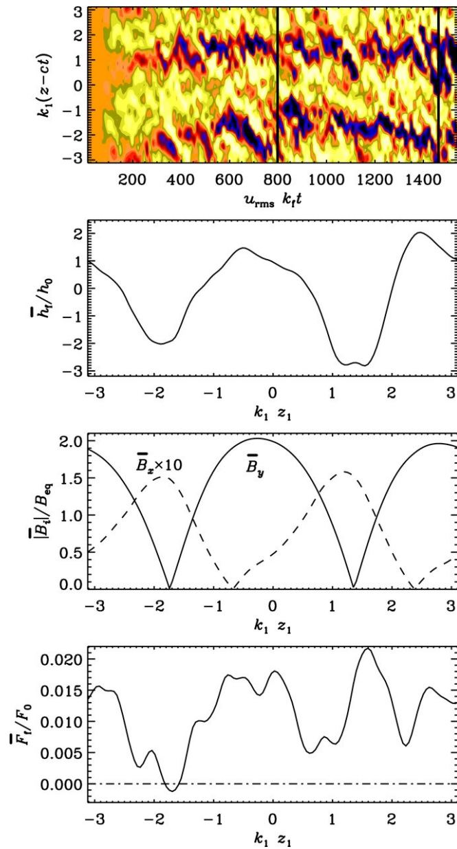
Figure 4. from Magnetic Helicity Flux in the Presence of Shear Hubbard & Brandenburg 2011 ApJ 727 11 doi:10.1088/0004-637X/727/1/11 https://dx.doi.org/10.1088/0004-637X/727/1/11 © 2011. The American Astronomical Society. All rights reserved.
