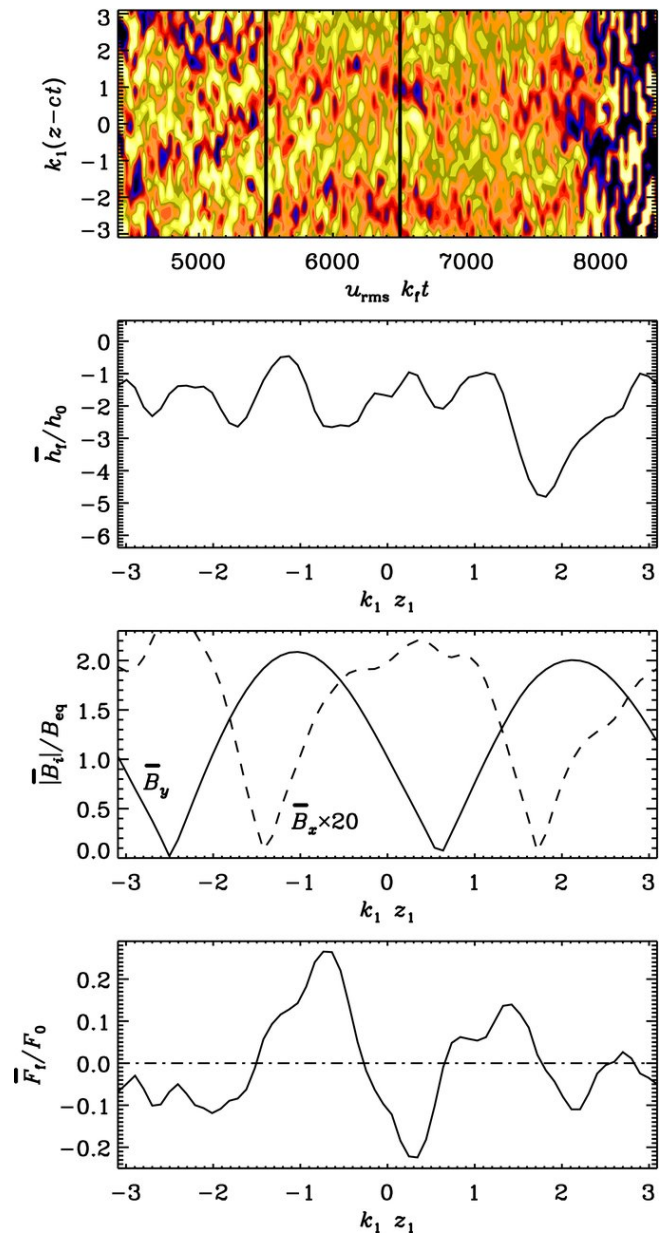
Figure 3. from Magnetic Helicity Flux in the Presence of Shear Hubbard & Brandenburg 2011 ApJ 727 11 doi:10.1088/0004-637X/727/1/11 https://dx.doi.org/10.1088/0004-637X/727/1/11 © 2011. The American Astronomical Society. All rights reserved.
