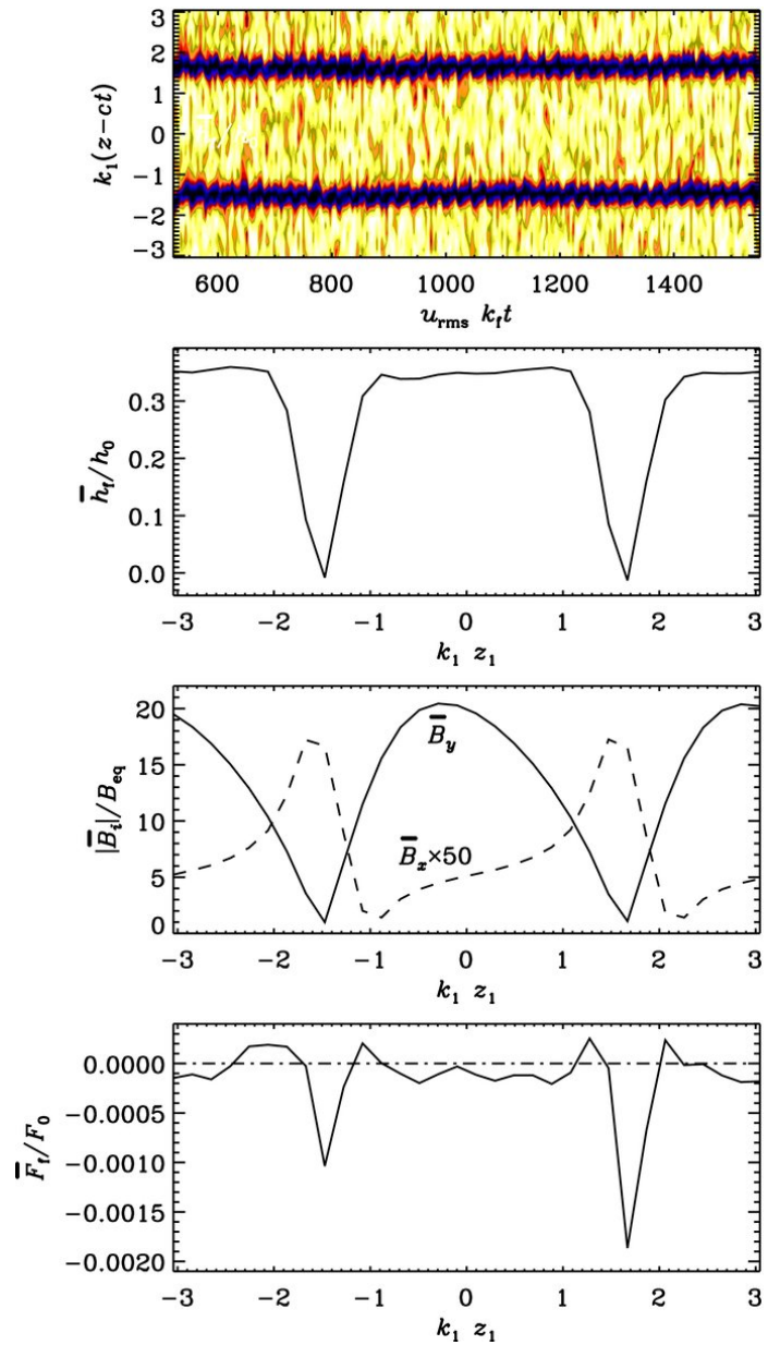
Figure 2. from Magnetic Helicity Flux in the Presence of Shear Hubbard & Brandenburg 2011 ApJ 727 11 doi:10.1088/0004-637X/727/1/11 https://dx.doi.org/10.1088/0004-637X/727/1/11 © 2011. The American Astronomical Society. All rights reserved.
