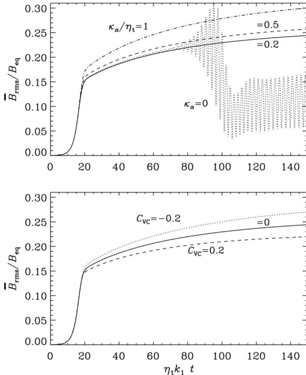
Figure 1. from Magnetic Helicity Flux in the Presence of Shear Hubbard & Brandenburg 2011 ApJ 727 11 doi:10.1088/0004-637X/727/1/11 https://dx.doi.org/10.1088/0004-637X/727/1/11 © 2011. The American Astronomical Society. All rights reserved.
