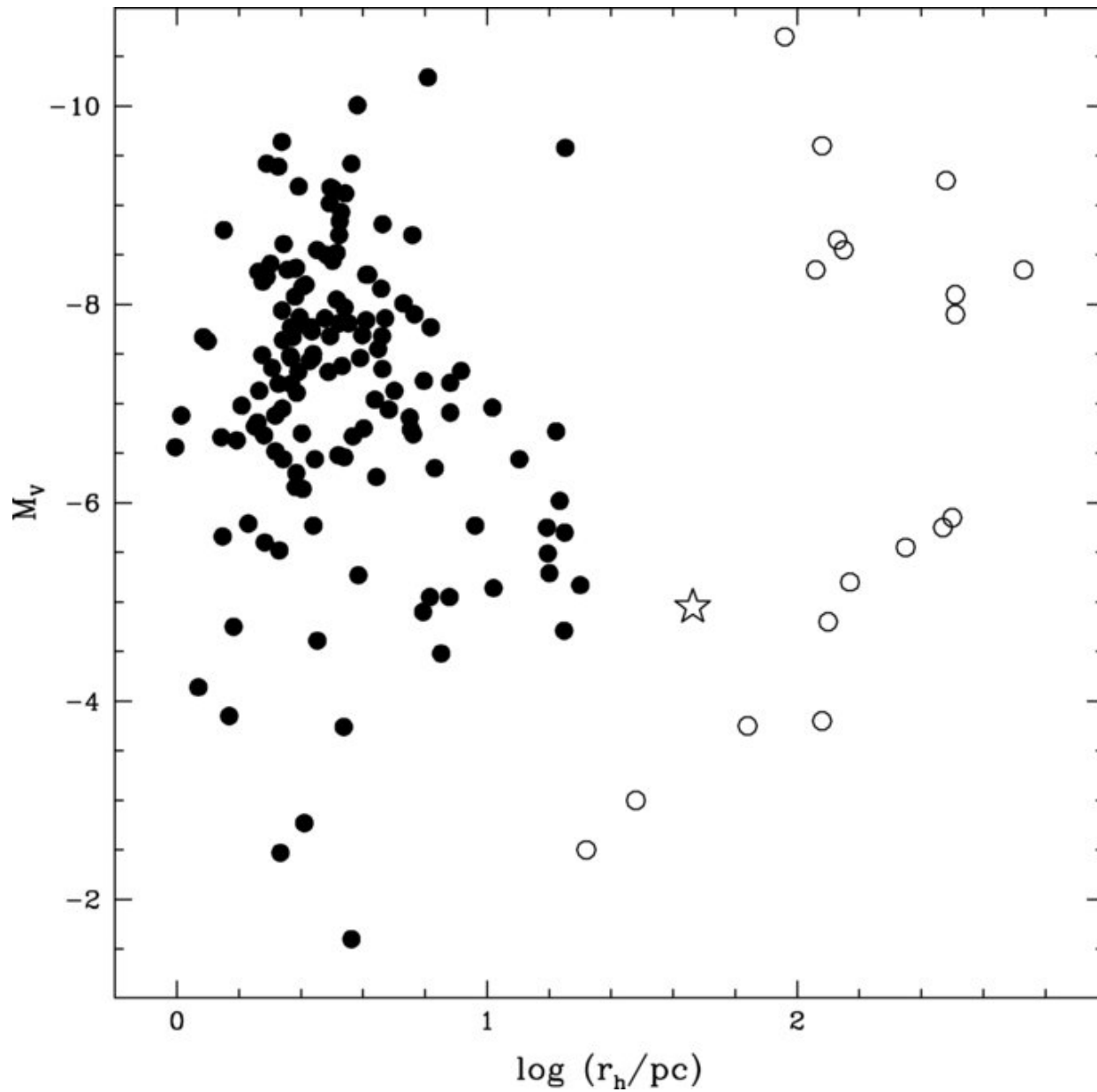
Figure 9. from Discovery of Tidal Tails Around the Distant Globular Cluster Palomar 14 Sollima et al. 2011 ApJ 726 47 doi:10.1088/0004-637X/726/1/47 https://dx.doi.org/10.1088/0004-637X/726/1/47 © 2011. The American Astronomical Society. All rights reserved.
