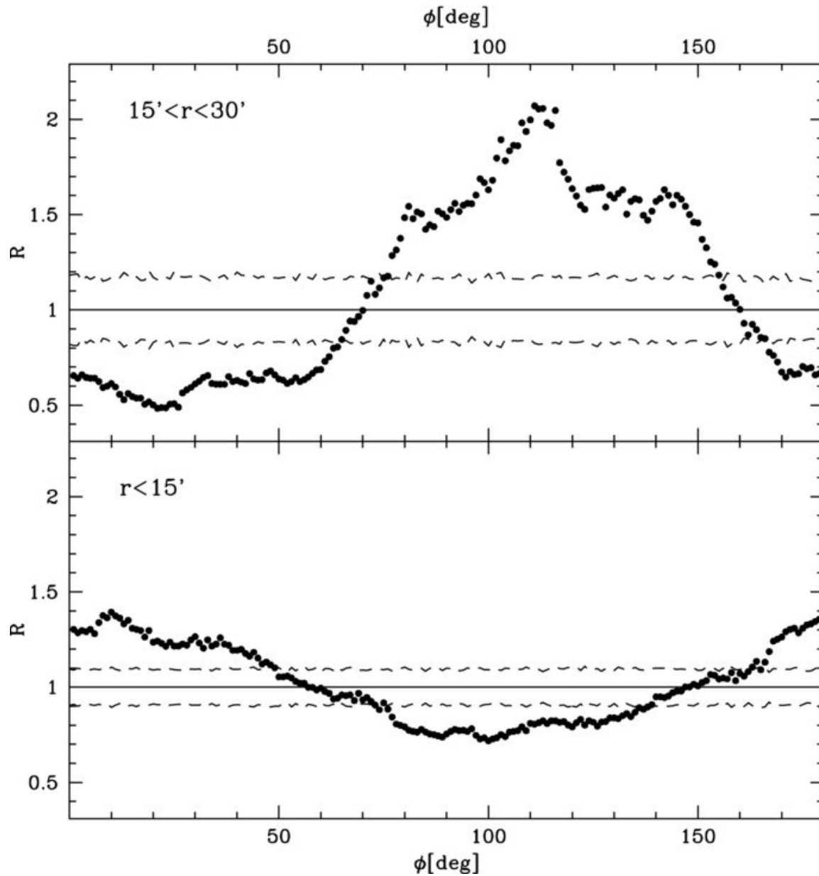
Figure 6. from Discovery of Tidal Tails Around the Distant Globular Cluster Palomar 14 Sollima et al. 2011 ApJ 726 47 doi:10.1088/0004-637X/726/1/47 https://dx.doi.org/10.1088/0004-637X/726/1/47 © 2011. The American Astronomical Society. All rights reserved.
