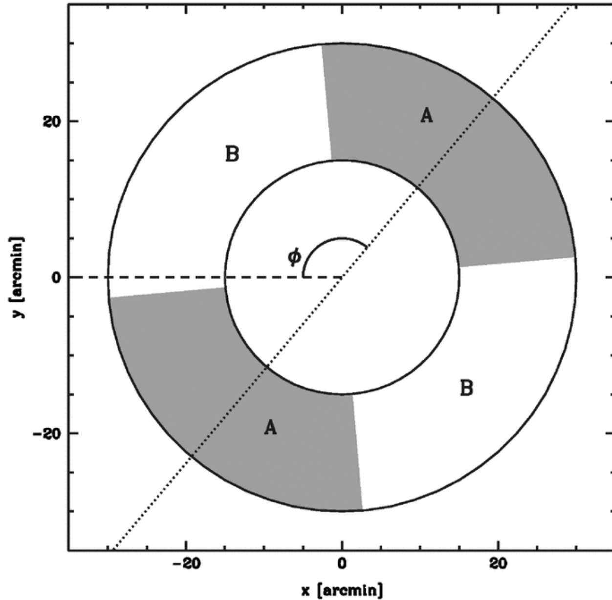
Figure 5. from Discovery of Tidal Tails Around the Distant Globular Cluster Palomar 14 Sollima et al. 2011 ApJ 726 47 doi:10.1088/0004-637X/726/1/47 https://dx.doi.org/10.1088/0004-637X/726/1/47 © 2011. The American Astronomical Society. All rights reserved.
