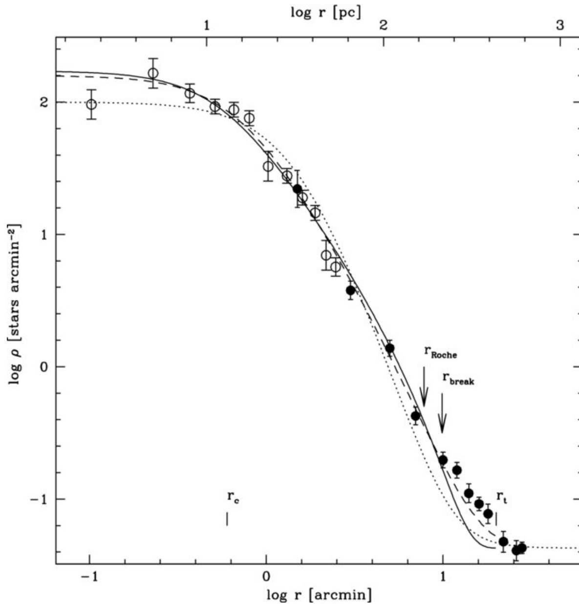
Figure 3. from Discovery of Tidal Tails Around the Distant Globular Cluster Palomar 14 Sollima et al. 2011 ApJ 726 47 doi:10.1088/0004-637X/726/1/47 https://dx.doi.org/10.1088/0004-637X/726/1/47 © 2011. The American Astronomical Society. All rights reserved.
