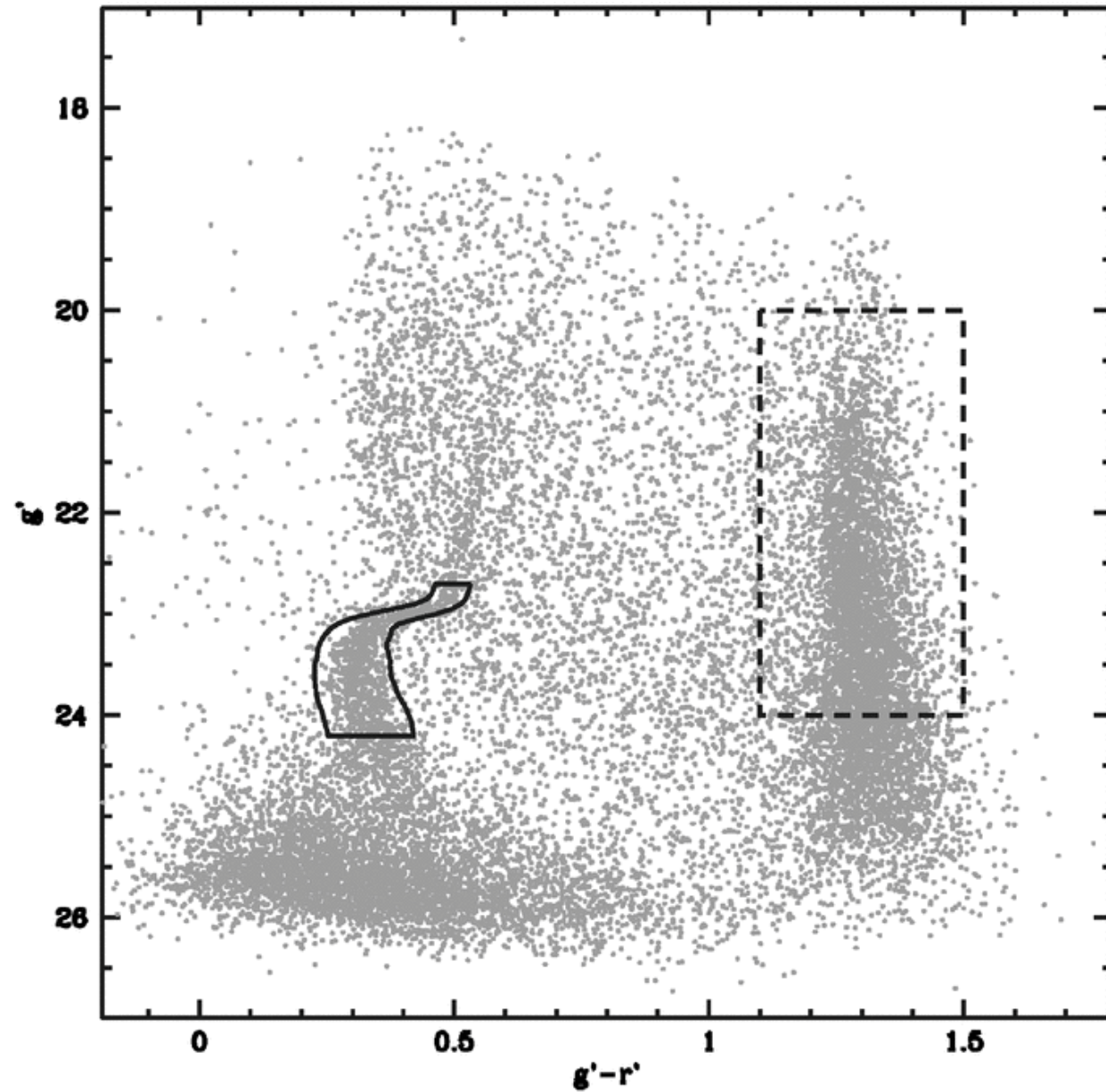
Figure 2. from Discovery of Tidal Tails Around the Distant Globular Cluster Palomar 14 Sollima et al. 2011 ApJ 726 47 doi:10.1088/0004-637X/726/1/47 https://dx.doi.org/10.1088/0004-637X/726/1/47 © 2011. The American Astronomical Society. All rights reserved.
