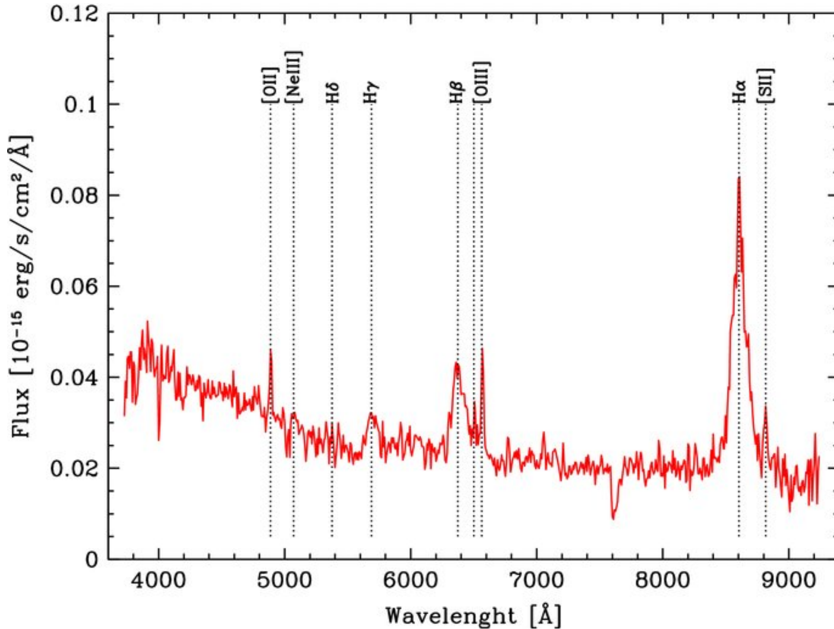
Figure 4. from Q2122-444: A Naked Active Galactic Nucleus Fully Dressed GLIOZZI ET AL. 2010 ApJ 725 2071 doi:10.1088/0004-637X/725/2/2071 https://dx.doi.org/10.1088/0004-637X/725/2/2071 © 2010. The American Astronomical Society. All rights reserved.
