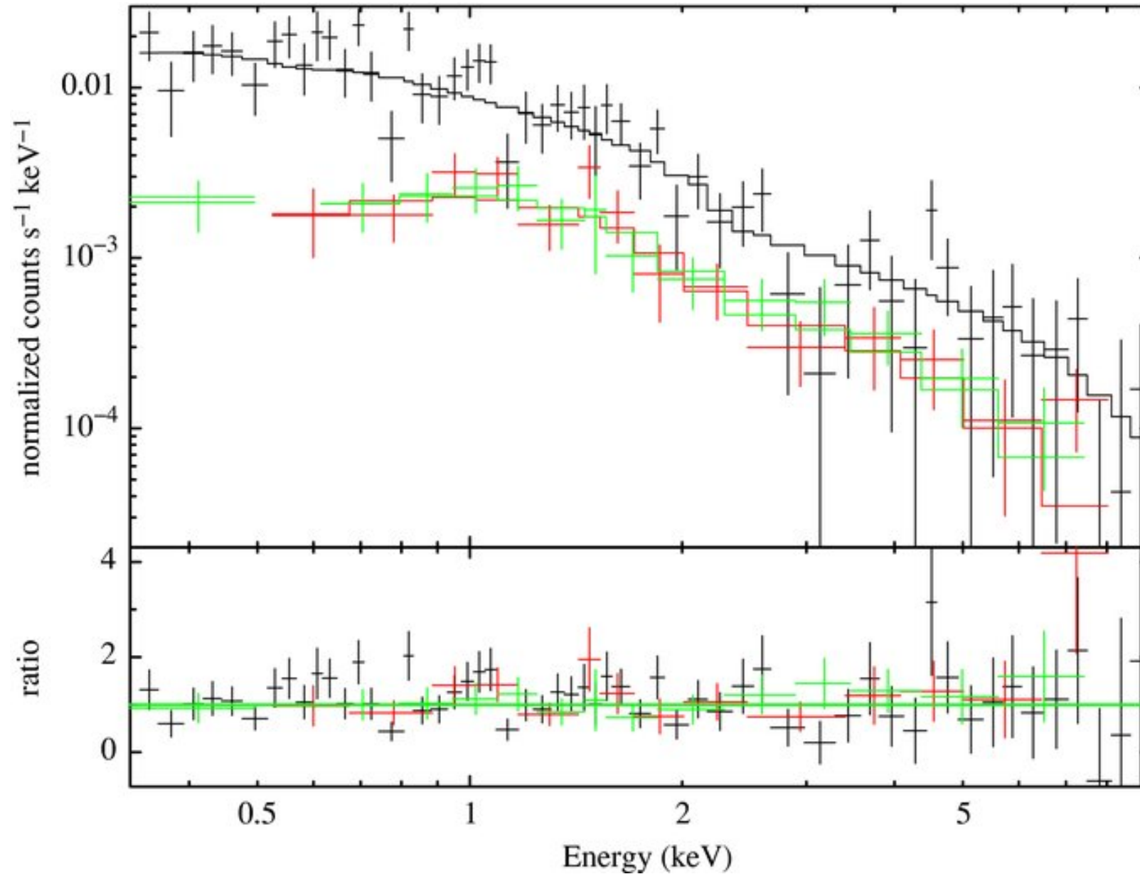
Figure 2. from Q2122-444: A Naked Active Galactic Nucleus Fully Dressed GLIOZZI ET AL. 2010 ApJ 725 2071 doi:10.1088/0004-637X/725/2/2071 https://dx.doi.org/10.1088/0004-637X/725/2/2071 © 2010. The American Astronomical Society. All rights reserved.
