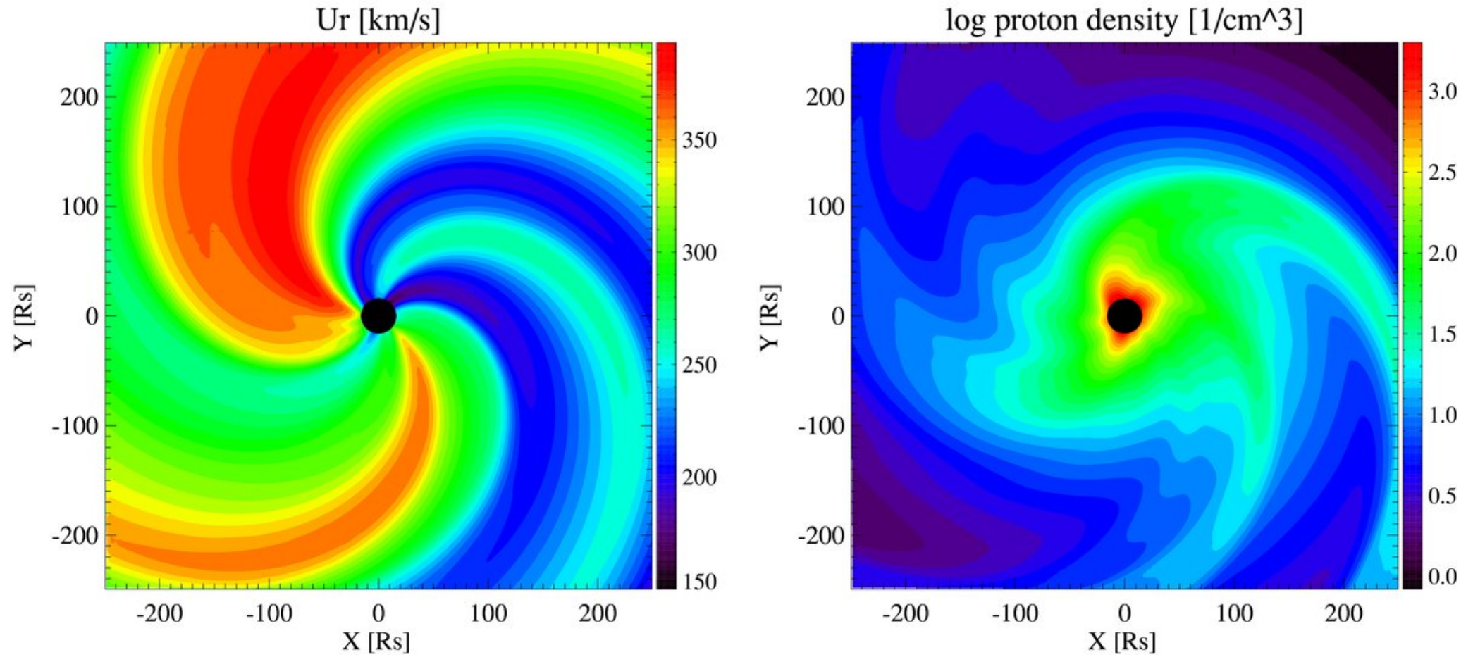
Figure 9. from A Data-driven, Two-temperature Solar Wind Model with Alfvén Waves VAN DER HOLST ET AL. 2010 ApJ 725 1373 doi:10.1088/0004-637X/725/1/1373 https://dx.doi.org/10.1088/0004-637X/725/1/1373 © 2010. The American Astronomical Society. All rights reserved.
