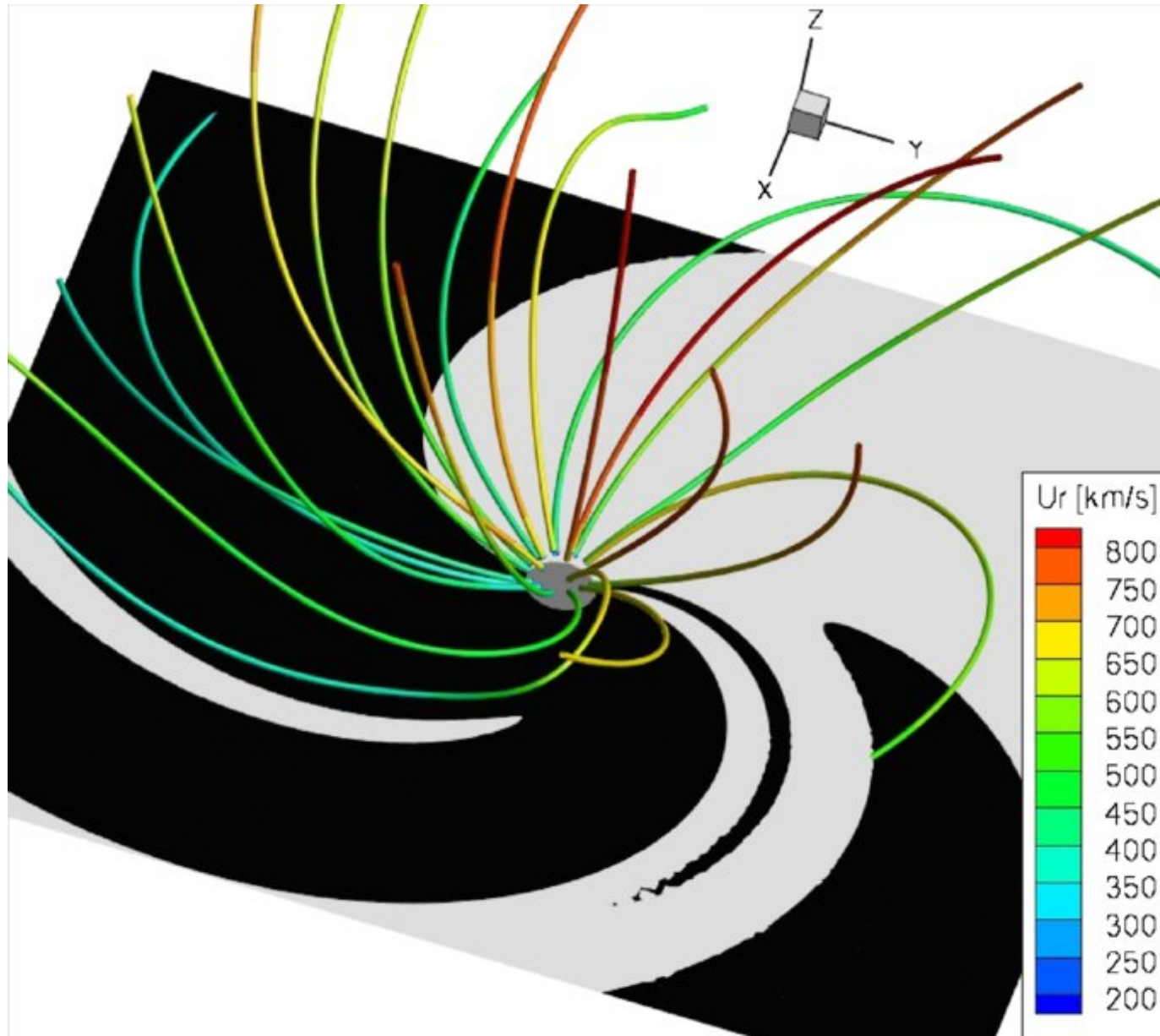
Figure 8. from A Data-driven, Two-temperature Solar Wind Model with Alfvén Waves VAN DER HOLST ET AL. 2010 ApJ 725 1373 doi:10.1088/0004-637X/725/1/1373 https://dx.doi.org/10.1088/0004-637X/725/1/1373 © 2010. The American Astronomical Society. All rights reserved.
