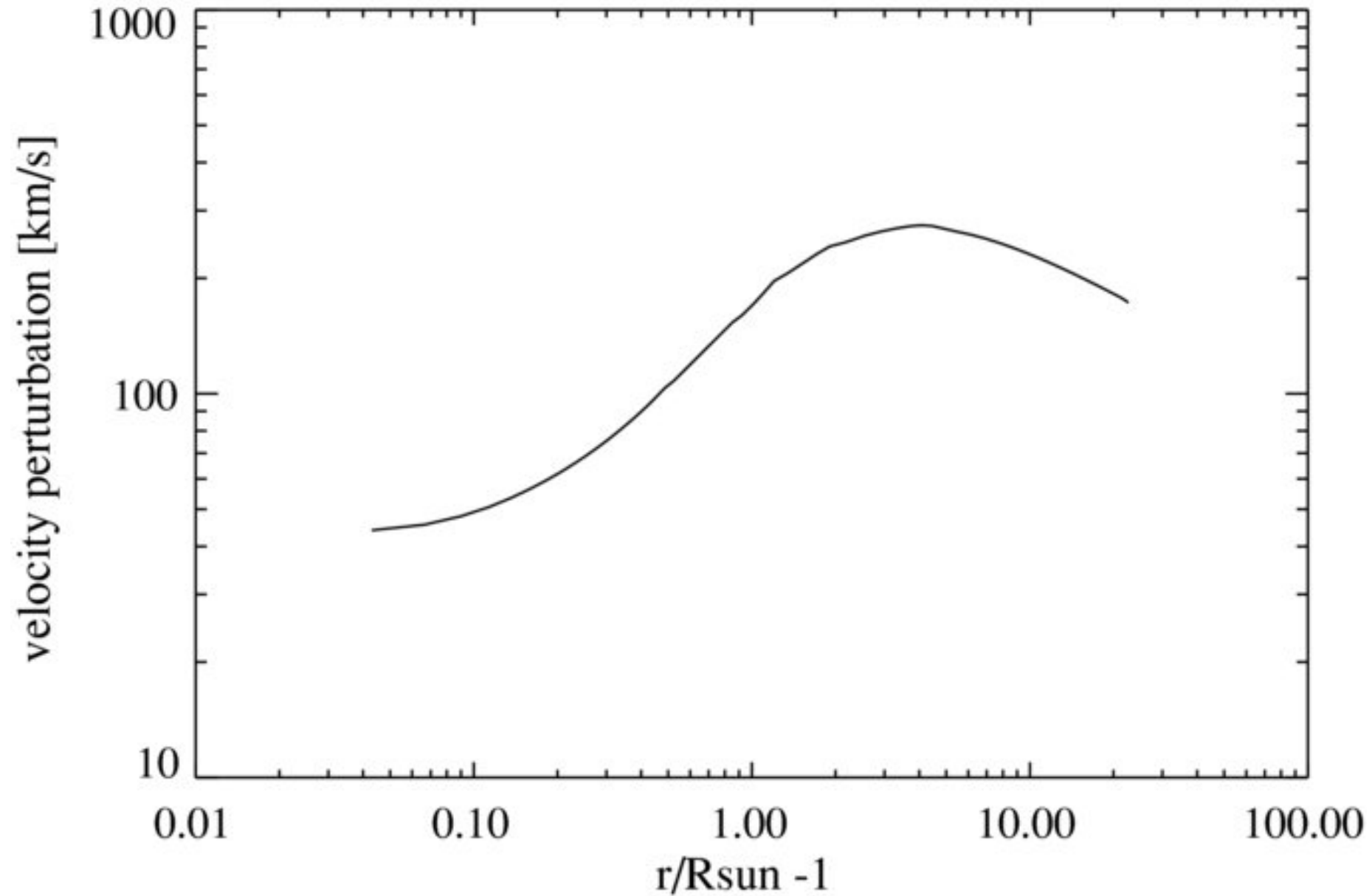
Figure 7. from A Data-driven, Two-temperature Solar Wind Model with Alfvén Waves VAN DER HOLST ET AL. 2010 ApJ 725 1373 doi:10.1088/0004-637X/725/1/1373 https://dx.doi.org/10.1088/0004-637X/725/1/1373 © 2010. The American Astronomical Society. All rights reserved.
