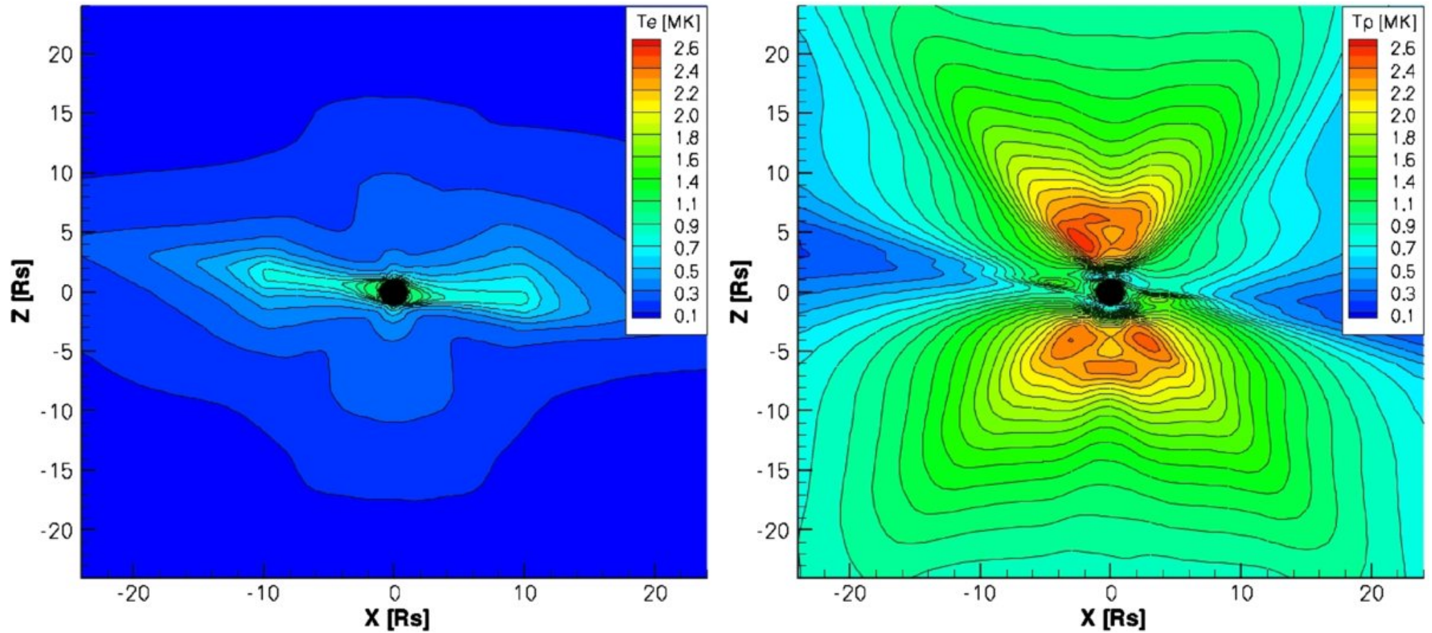
Figure 6. from A Data-driven, Two-temperature Solar Wind Model with Alfvén Waves VAN DER HOLST ET AL. 2010 ApJ 725 1373 doi:10.1088/0004-637X/725/1/1373 https://dx.doi.org/10.1088/0004-637X/725/1/1373 © 2010. The American Astronomical Society. All rights reserved.
