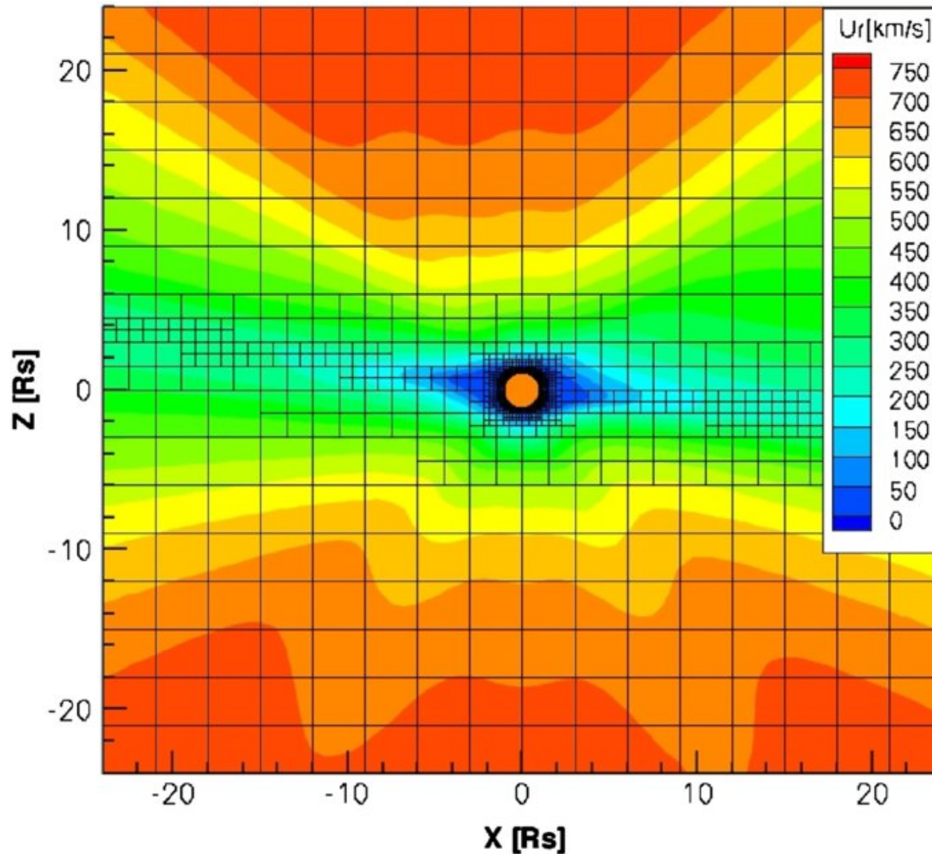
Figure 5. from A Data-driven, Two-temperature Solar Wind Model with Alfvén Waves VAN DER HOLST ET AL. 2010 ApJ 725 1373 doi:10.1088/0004-637X/725/1/1373 https://dx.doi.org/10.1088/0004-637X/725/1/1373 © 2010. The American Astronomical Society. All rights reserved.
