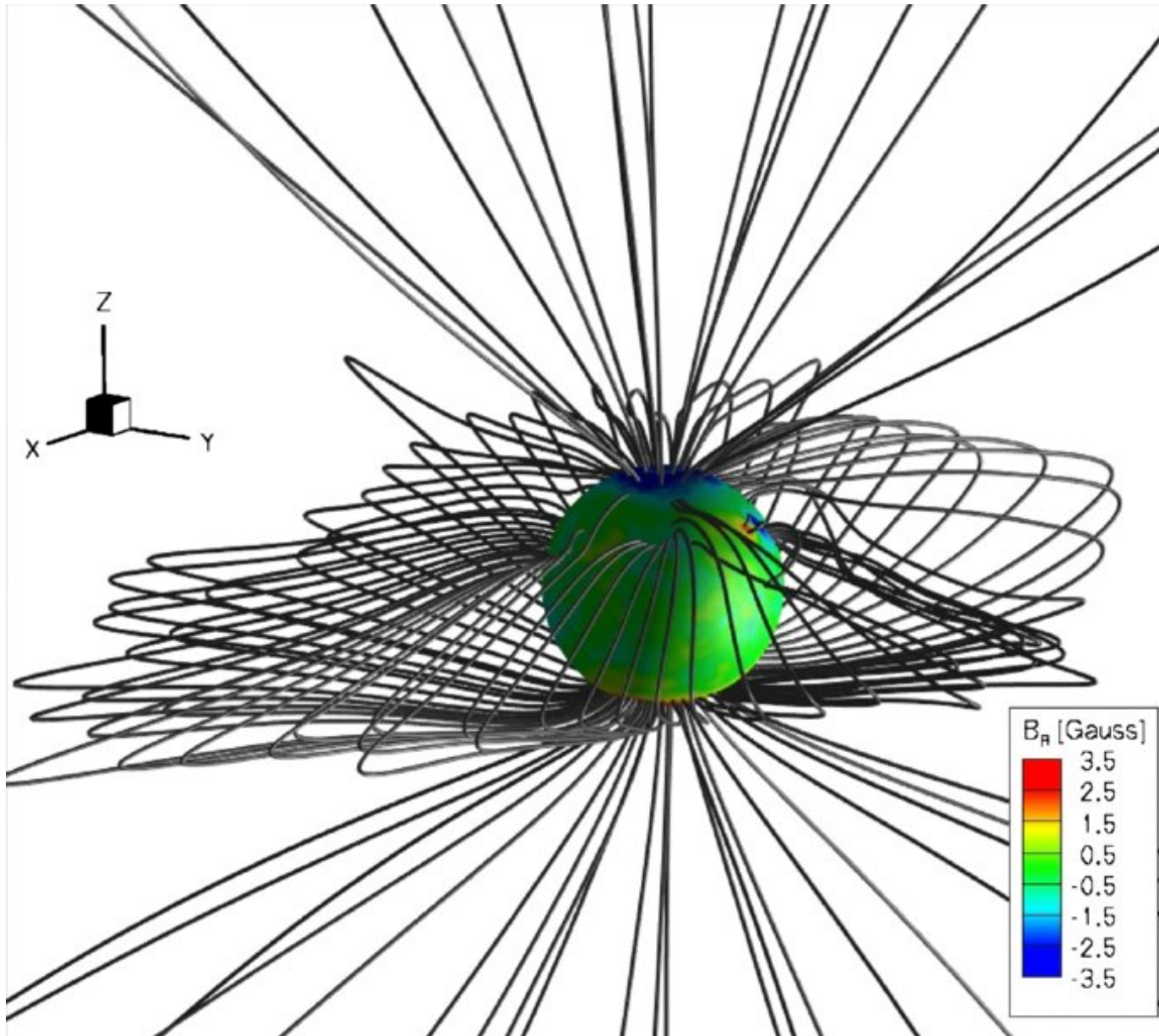
Figure 4. from A Data-driven, Two-temperature Solar Wind Model with Alfvén Waves VAN DER HOLST ET AL. 2010 ApJ 725 1373 doi:10.1088/0004-637X/725/1/1373 https://dx.doi.org/10.1088/0004-637X/725/1/1373 © 2010. The American Astronomical Society. All rights reserved.
