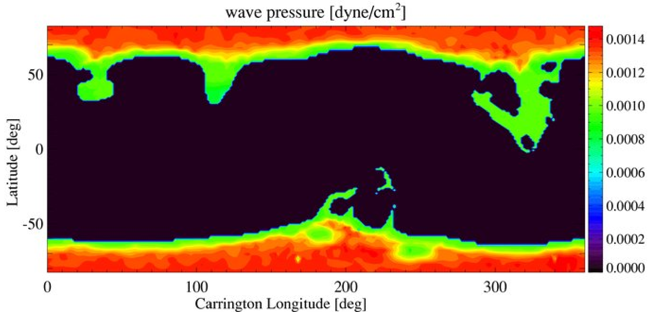
Figure 3. from A Data-driven, Two-temperature Solar Wind Model with Alfvén Waves VAN DER HOLST ET AL. 2010 ApJ 725 1373 doi:10.1088/0004-637X/725/1/1373 https://dx.doi.org/10.1088/0004-637X/725/1/1373 © 2010. The American Astronomical Society. All rights reserved.
