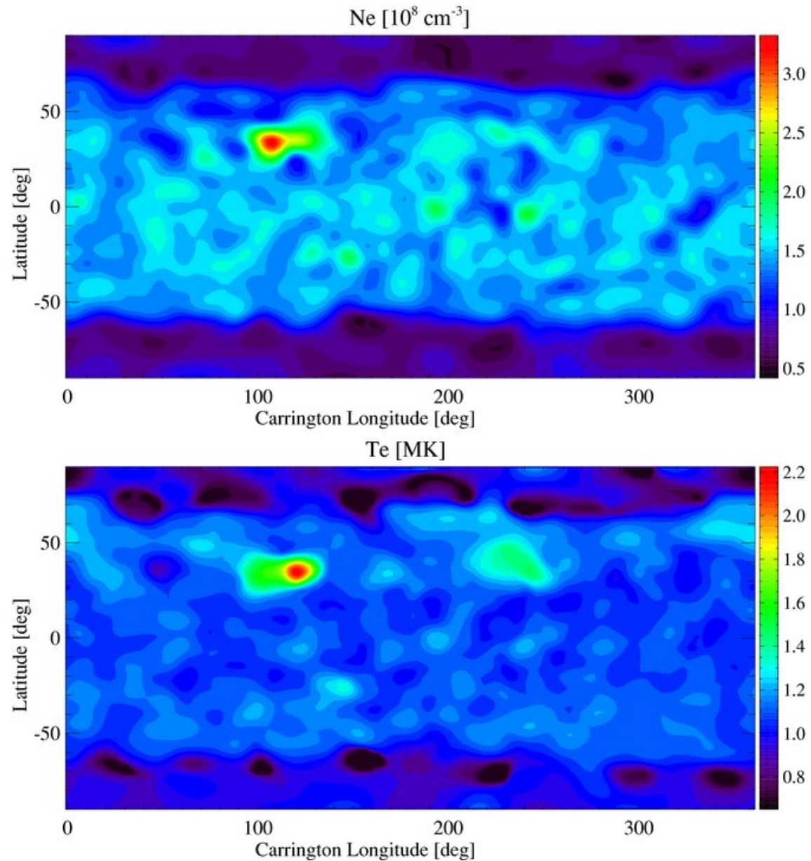
Figure 2. from A Data-driven, Two-temperature Solar Wind Model with Alfvén Waves VAN DER HOLST ET AL. 2010 ApJ 725 1373 doi:10.1088/0004-637X/725/1/1373 https://dx.doi.org/10.1088/0004-637X/725/1/1373 © 2010. The American Astronomical Society. All rights reserved.
