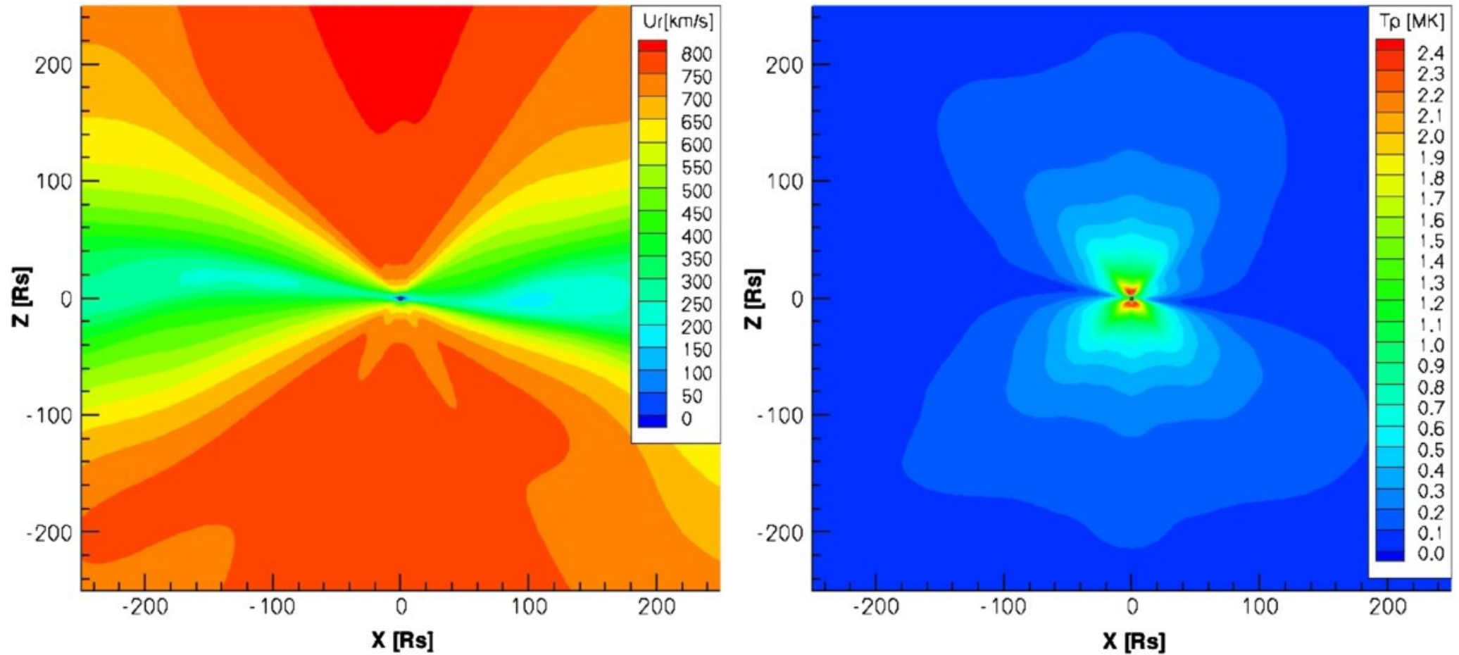
Figure 11. from A Data-driven, Two-temperature Solar Wind Model with Alfvén Waves VAN DER HOLST ET AL. 2010 ApJ 725 1373 doi:10.1088/0004-637X/725/1/1373 https://dx.doi.org/10.1088/0004-637X/725/1/1373 © 2010. The American Astronomical Society. All rights reserved.
