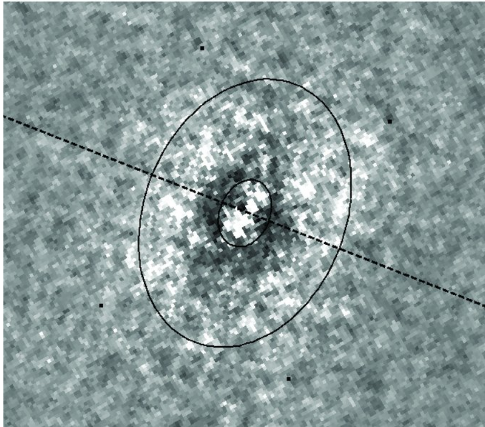
Figure 4. from Gas Accretion in the M32 Nucleus: Past and Present SETH 2010 ApJ 725 670 doi:10.1088/0004-637X/725/1/670 https://dx.doi.org/10.1088/0004-637X/725/1/670 © 2010. The American Astronomical Society. All rights reserved.
