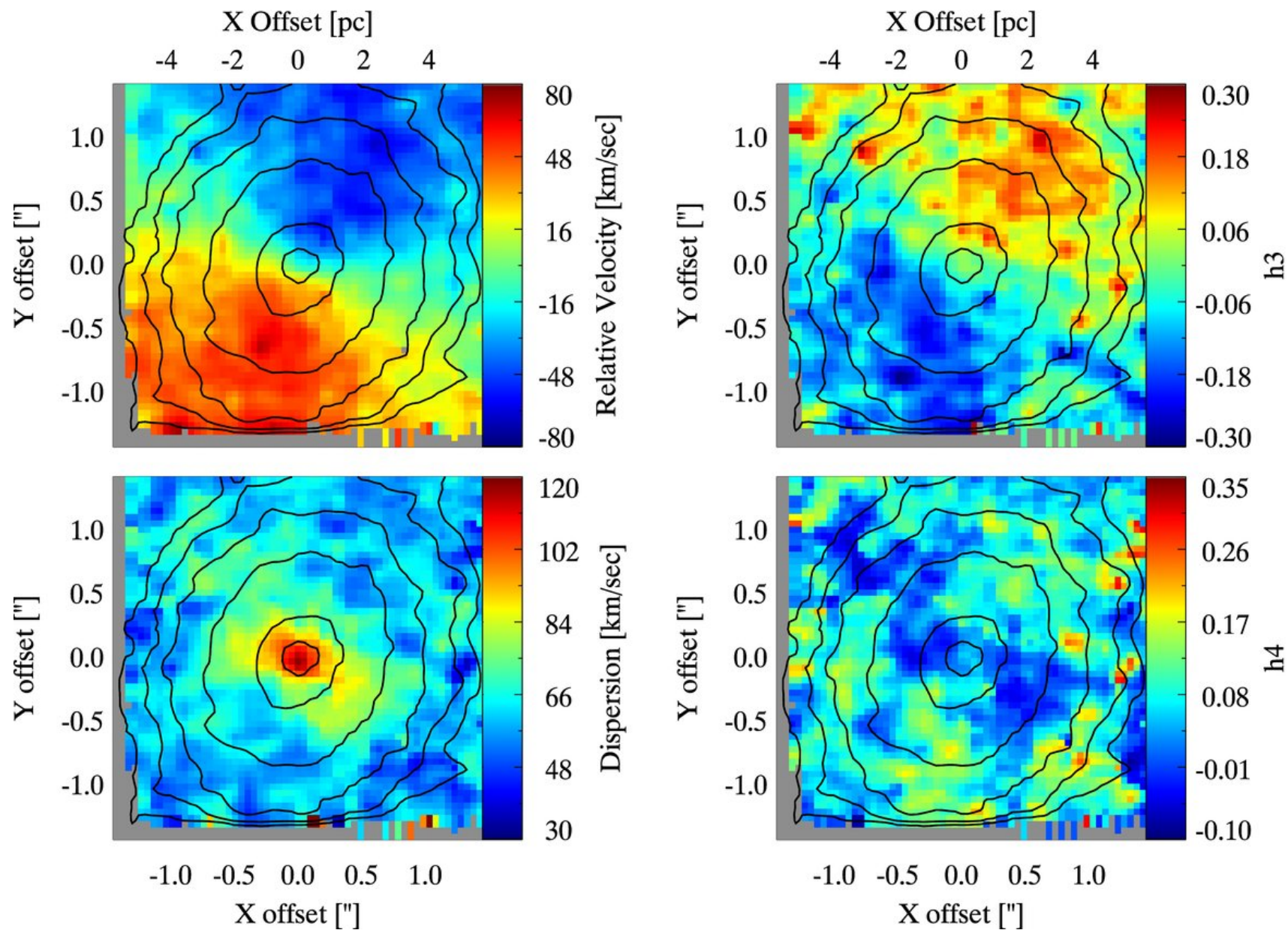
Figure 2. from Gas Accretion in the M32 Nucleus: Past and Present SETH 2010 ApJ 725 670 doi:10.1088/0004-637X/725/1/670 https://dx.doi.org/10.1088/0004-637X/725/1/670 © 2010. The American Astronomical Society. All rights reserved.
