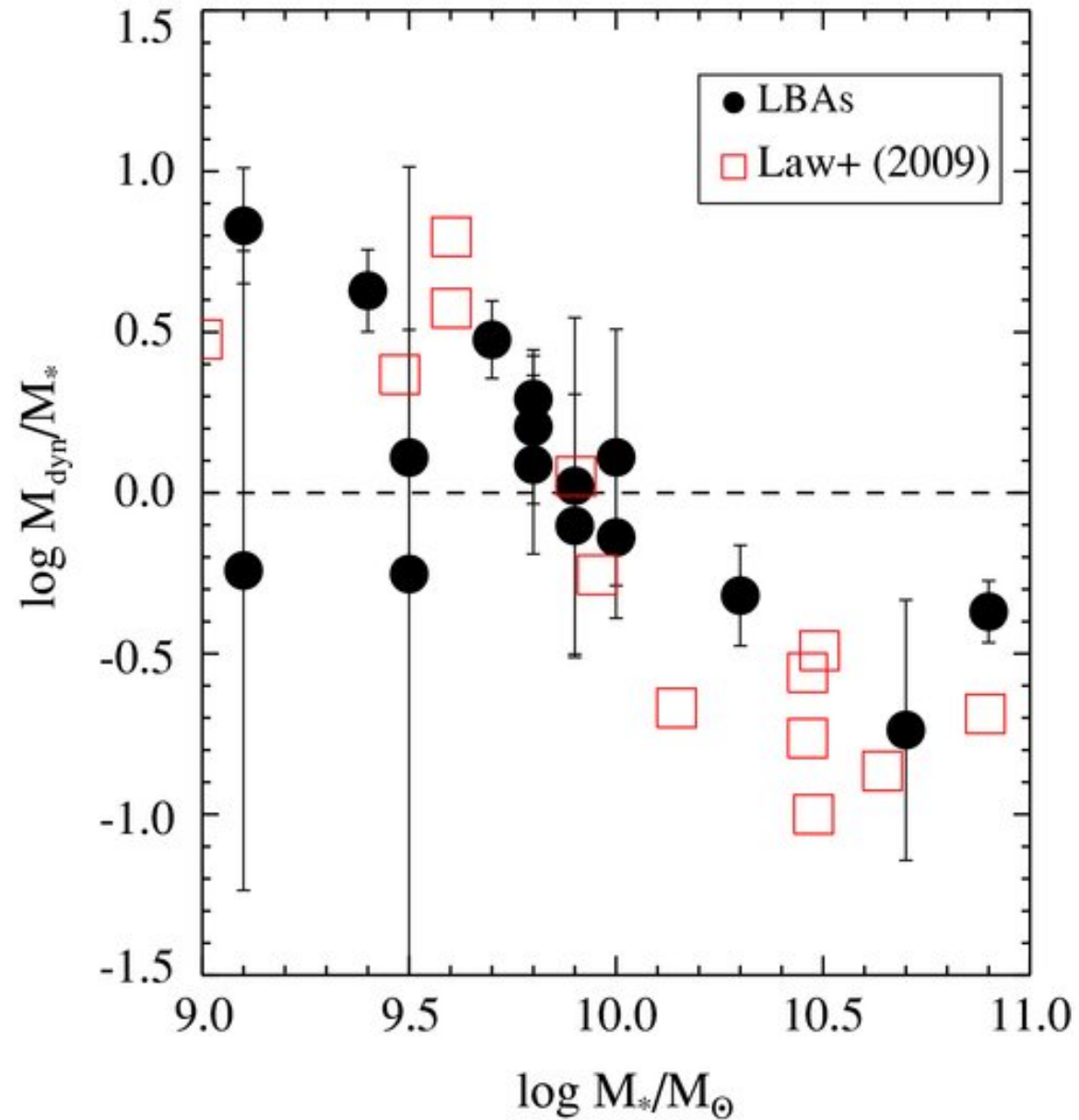
Figure 6. from The Kinematics of Ionized Gas in Lyman-break Analogs at z \sim 0.2 GONÇALVES ET AL. 2010 ApJ 724 1373 doi:10.1088/0004-637X/724/2/1373 https://dx.doi.org/10.1088/0004-637X/724/2/1373 © 2010. The American Astronomical Society. All rights reserved.
